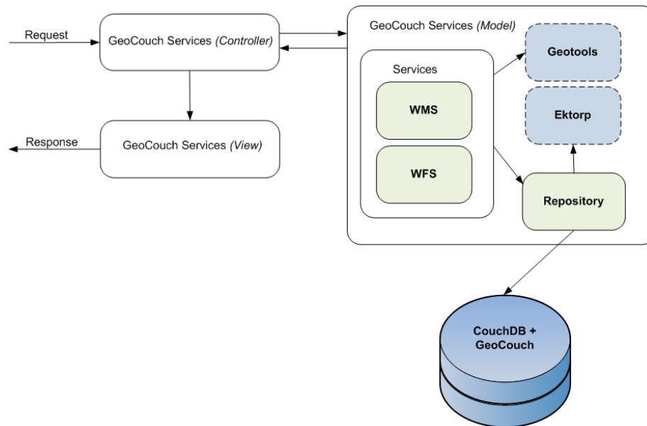
Figure 2: GeoCouchServices MVC architecture.
