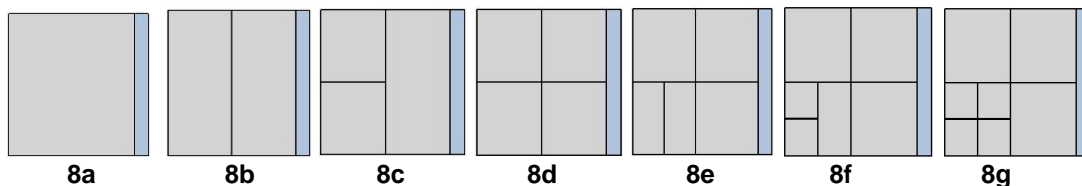
Figure 8. Extent partitioning
