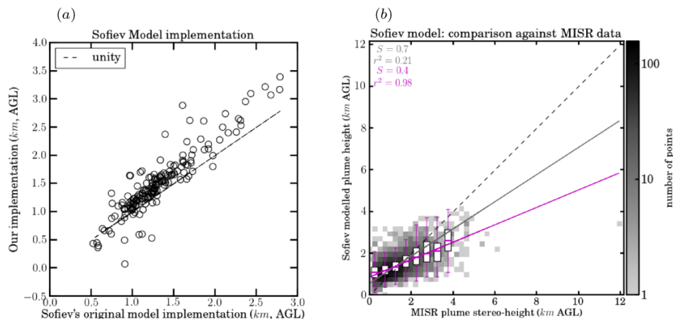
Figure 7. Comparison of our implementation of the plume rise parameterization of Sofiev et al. (2012) to (a) the original results from Sofiev et al. (2012) for the same fires and (b) plume stereo-height retrievals extracted from the North American subset of the (MISR) plume height project data Nelson et al. (2013), derived using the MINX tool as shown in Fig. 4. Our implementation of the Sofiev et al. (2012) model differs from the original in its definition of the PBL height, which in our approach is extracted from the diagnostic product of ECMWF forecast runs (ECMWF, 2012). See Figs. 9 and 10 for a statistical overview of the North American MISR data set. Note that the Sofiev et al. (2012) model did not retrieve simulated plume heights for all the 3320 selected fires of that data set. For 114 fires, either the Brunt–Väisälä frequency could not be retrieved or the FRP of the most powerful pixel listed in the MISR product was unavailable (see Sofiev et al., 2012, for details in the initialization of the model). Panel (b) shows the same metrics as Fig. 2 of Val Martin et al. (2012), i.e. two-sided regression line (grey), box plots of the distributions of model heights and 500 m resolution MISR heights for central 67 % (box) and central 90 % (cap), median distribution regression line (magenta), and 1 : 1 relationship (dashed black).
