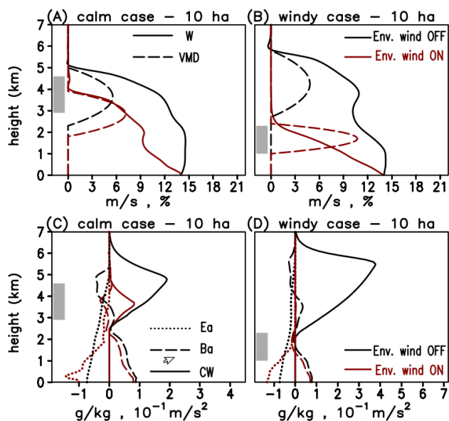
Figure 5. Results from the one-dimensional plume rise model (PRM) of Freitas et al. (2007, 2010) for a fire burning in (a, c) calm and (b, d) windy atmosphere scenario, as studied by Freitas et al. (2010). The fire has an active fire area (AF area) of 10 ha. The quantities shown are vertical velocity ( W , \text{ms}^{-1} ), vertical mass distribution (VMD, %), entrainment acceleration ( E_a , 10^{-1} \text{ms}^{-2} ), buoyancy acceleration ( B_a , 10^{-1} \text{ms}^{-2} ), and total condensate water ( CW , \text{g kg}^{-1} ). Model results considering the environmental wind drag are shown in red, whilst those in black depicts the results from simulations disregarding this effect. Grey rectangles indicate the main injection height simulated by the three-dimensional ATHAM model (Trentmann et al., 2006) for the same fire scenario. Figure from Freitas et al. (2010).
