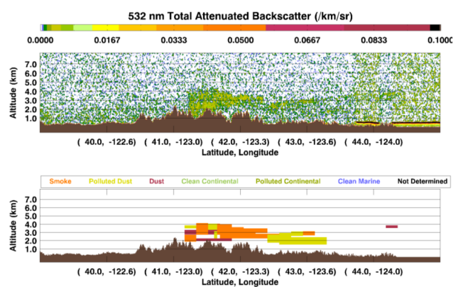
Figure 3. Example of profiles for Level-1 CALIOP 532 nm total attenuated backscatter data product (top) and the matching Level-2 product of aerosol layers (bottom) for the 28 August 2006 over the Klamath Mountains in California and Oregon. The presence of aerosols classified as biomass burning smoke can be seen. Image from Raffuse et al. (2012).
