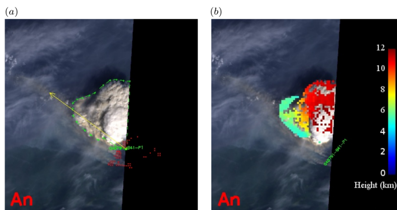
Figure 11. Overview of the highest fire plumes present in the current North American subset of the MISR plume height data set of Nelson et al. (2013), derived using the MINX tool shown in Fig. 4. The reference of this fire in the MISR data set is O45791-B41-P1, and it was observed in the Northwest Territories (Canada) on 27 July 2008. It shows the nadir image recorded by MISR, together with the plume contour set by the operator of the MINX software (a), the estimated wind direction (yellow arrow in a), and the stereo-height retrieval (b). Part of the image is black as the fire was located on the edge of the MISR swath. Images are taken from the MISR plume height project website (see footnote 1).
