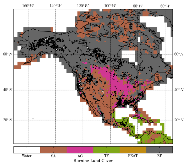
Figure 9. Fire locations contained within the Multi-angle Imaging SpectroRadiometer (MISR) plume height data set of Nelson et al. (2013) over North America for the time period 2001–2008 (black dots). White dots indicate the locations of the 22 fires plumes classed as having a plume height in excess of 4.5 km. The map in the background shows the land cover used within the GFEDv3 biomass burning emissions inventory of van der Werf et al. (2010) where SA, AG, TF, PEAT, and EF stand for savannah, agriculture, tropical forest, peat land, and extra tropical forest respectively.
