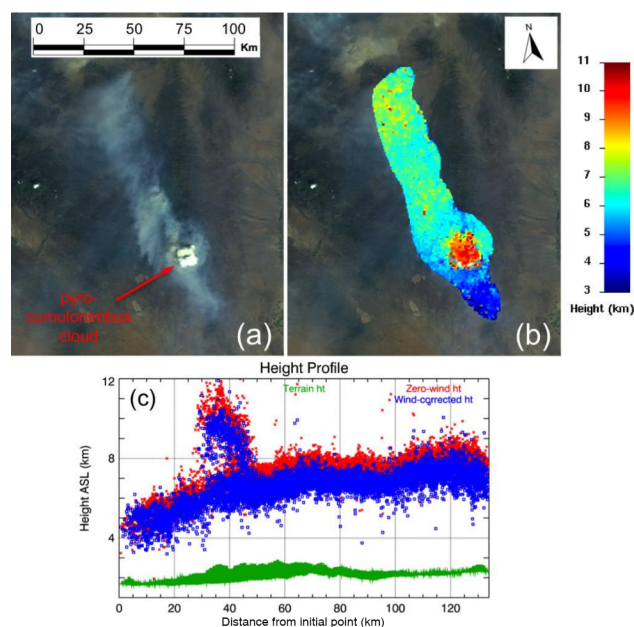
Figure 4. Example of smoke plume height derivation using data from the Multiangle Imaging SpectroRadiometer (MISR) that operates on the Terra satellite. This example is extracted from Nelson et al. (2013). The fire took place on the 12 July 2013 in New Mexico and was observed by MISR at 18:09 UTC. The MISR nadir RGB image showing a smoke plume in grey and a PyroCb in bright white is reported in (a), when the plume stereo-heights derived from the MINX software (Nelson et al., 2013) are shown in (b). MINX height retrieval profiles are shown in (c). Note the dramatic difference in the heights which reach 11–12 km a.s.l. in the PyroCb and stay trapped in a layer around 6–8 km a.s.l. in the vicinity.
