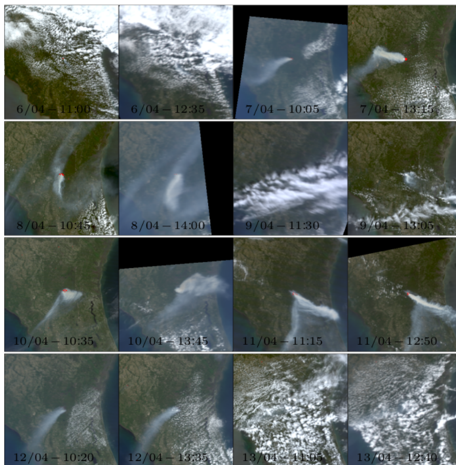
Figure 1. True colour composite of daytime observations of the county fire (USA), made from the Moderate Resolution Imaging Spectroradiometer (MODIS) satellite EO sensor. The fire occurred in Ocala National Forest (Florida) between 5 and 13 April 2012. MODIS data from all available Terra and Aqua satellite overpasses are shown, with the local time indicated. Overlain on the colour composite imagery are red vectors that outline pixels detected as containing active fires by the MODIS MOD14/MYD14 Active Fire and Thermal Anomaly Products (Giglio et al., 2003). The regularly changing nature of the fire and the smoke transport apparent from this time series, as well as the presence on some days of bifurcated plumes, is very apparent.
