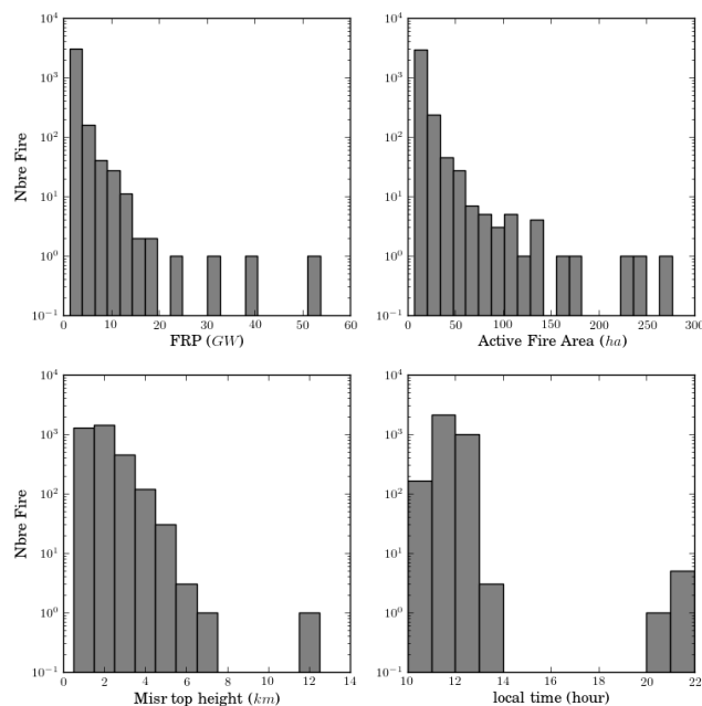
Figure 10. Distribution of FRP (a), active fire area (b), top plume height (c), and local time observation (d) for the 3320 fires of the current North American subset of the Multi-angle Imaging Spectro-Radiometer (MISR) plume height project data set of Nelson et al. (2013) derived using the MINX tool shown in Fig. 4.
