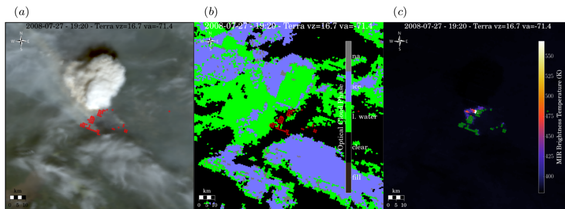
Figure 12. Images from the wider-swath Moderate Resolution Imaging Spectroradiometer (MODIS) for the same fire as in Fig. 11 at the same time. MODIS is mounted on the same Terra satellite as MISR (see Sect. 4.1). (a) is the false colour composite image of the area observed. (b) is the Middle Infra-Red brightness temperature. (c) is the optical cloud phase properties of the version 6 of the MODIS cloud product Platnick et al. (2003). Cross markers in (a) and (c) (red and green respectively) denote the location of MODIS pixels detected as containing active fire in the MODIS MOD14 active fire product of Giglio et al. (2003).
