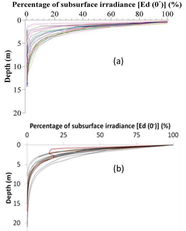
Fig. 2 Downwelling irradiance decay with depth: (a) in Tucuruí and (b) Três Marias reservoir.
