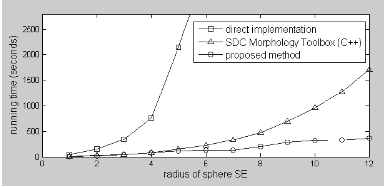
Figure 9. Processing times for gray-level dilation (binary SE) using sphere SE for a 512 \times 512 \times 418 chest CT image. Results obtained on Intel Pentium IV Xeon Dual CPU 2.00 GHz platform with 2.00 GB of RAM.
