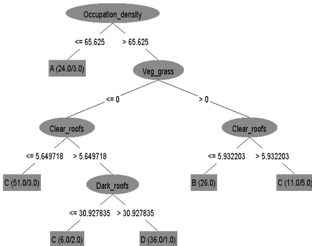
Fig. 7 - Decision tree obtained by selected features at WEKA.
