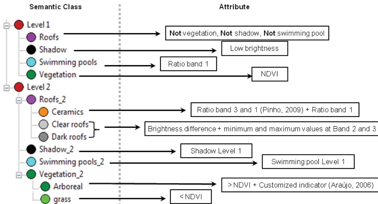
Fig. 4 – Semantic net and attributes used for image classification.
