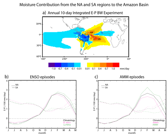
Figure 2. (a) Climatological annual average of 10-day integrated ( E - P ) obtained through the backward Amazon experiment for the period June 1979–May 2012. The black contour line indicates the basin area, and the boxes NA and SA indicate the source areas selected. (b) The annual cycle of the monthly values of 10-day ( E - P ) shown in Fig. 1 and integrated over the NA (continuous line) and SA (traced line) source areas indicated in (a). Black lines represent the 33-year average values, while pink and green lines indicate the average of the El Niño and La Niña events, respectively. (c): as (b), but the pink and green lines indicate the average of the AMM+ and AMM– events, respectively.
