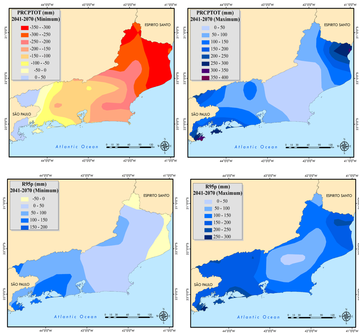
Figure 7. Minimum (left) and maximum differences (right) between the future (2041-2070) and present (1961-1990) indicators PRCPTOT (above) and R95p (below) in mm.
