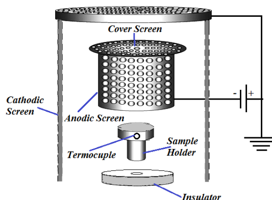
Fig. 1. Schematic representation of active screen system
