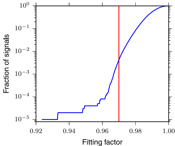
FIG. 2. Cumulative distribution of fitting factors obtained with the template bank for a population of simulated aligned-spin binary black hole signals. Less than 1% of the signals have a matched-filter SNR loss greater than 3%, demonstrating that the template bank has good coverage of the target search space.
