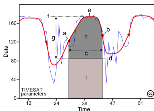
Figure 5. Some of the seasonality parameters generated by TIMESAT: (a) beginning of season, (b) end of season, (c) length of season, (d) base value, (e) time of middle of season, (f) maximum value, (g) amplitude, (h) small integrated value, (h+i) large integrated value. The red and blue lines represent the filtered and the original data, respectively.
