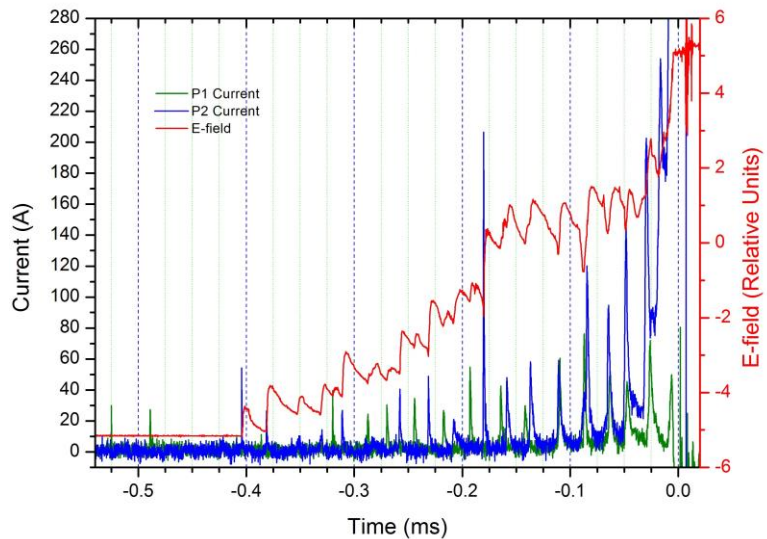
Fig. 5 – Measured current profile of a UCL from P1 and P2 (numbers 1 and 2) and from a UUL (numbers 3 to 6) from the side of P2 and from other buildings (see Fig. 1). The electric field was saturated before time t = -0.4 ms.
