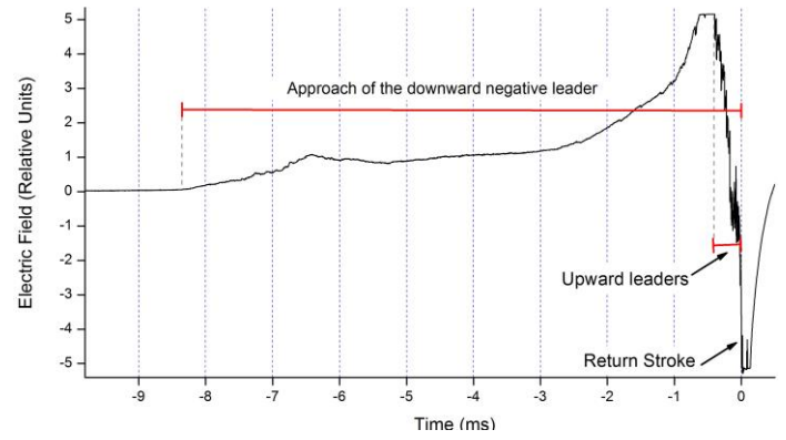
Fig. 4 – Electric field change with the approach of the negative downward leader and the initiation of the positive upward leaders.
