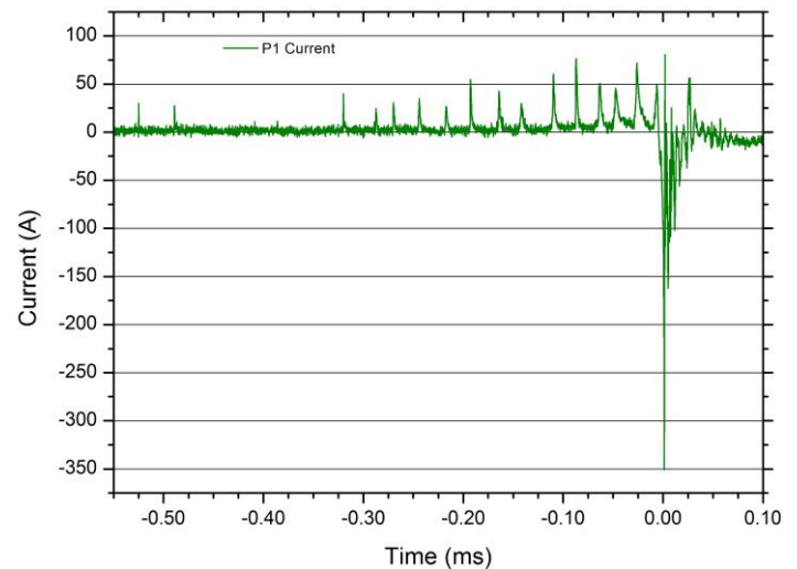
Fig. 6 – Current measurement of the UUL from P1 (leader number 1).
