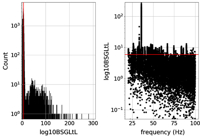
FIG. 7. Detection statistic of the loudest candidate from each stage 1 search: the distribution of their detection statistic values \hat{\beta}_{\text{S/GLL}} (left) and their distribution as a function of frequency (right). 411 candidates have \hat{\beta}_{\text{S/GLL}} values lower than the axes boundaries on the right plot. The red line marks \hat{\beta}_{\text{S/GLL}} = 6.0 which is the threshold at and above which candidates are passed on to stage 2.
