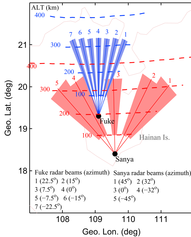
Figure 1. The Sanya and Fuke VHF radar beam directions projected on the geographic longitude-latitude plane. The shaded area in each direction represents the 3 dB (half power full beam) width.
