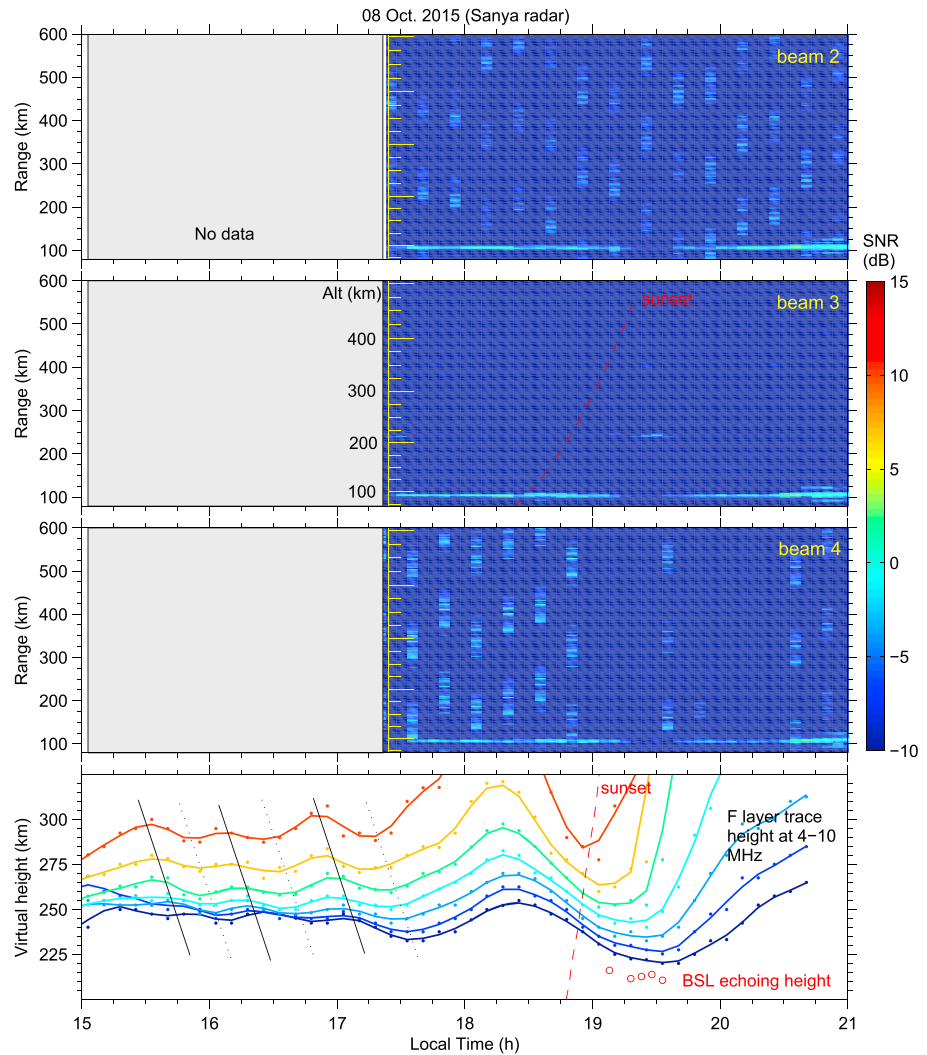
Figure 5. Sanya radar observations on 8 October 2015 (a geomagnetic disturbed day) when no obvious presunset BSL echoes detected. The fourth panel shows obvious F layer height oscillations observed for a long time, around 1530–1800 LT.
