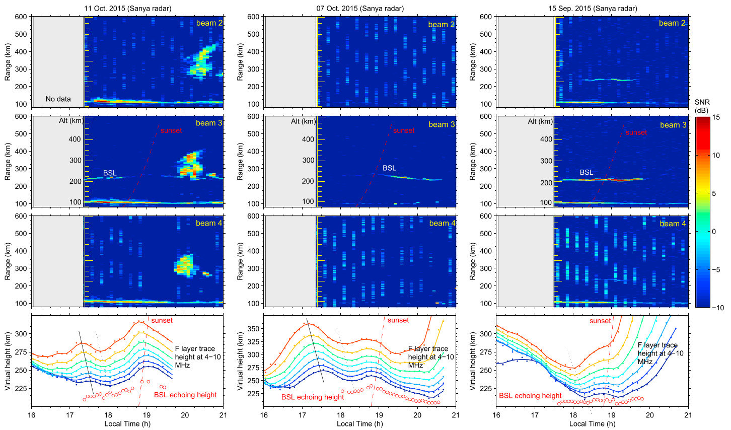
Figure 4. Three cases of presunset BSL observed by the Sanya radar on (left column) 11 October, (middle column) 7 October, and (right column) 15 September, 2015, respectively. Note that on 7 October the BSL echo intensity around 1800–1900 LT is very weak. The shaded area (gray) in the left of each RTI map indicates no F region observation. The bottom plots show F layer virtual heights at seven plasma frequencies from 4 to 10 MHz, with an interval of 1 MHz. The BSL echoing heights (shown as circles) are superimposed in the panels.
