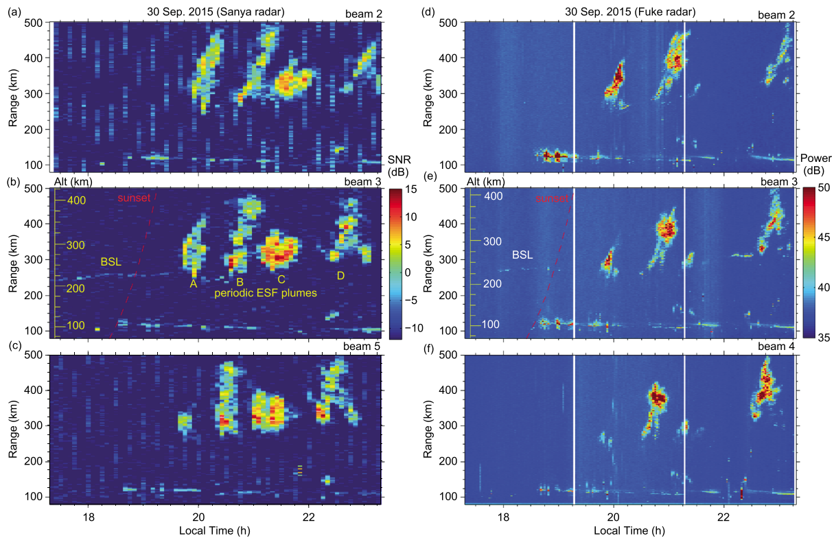
Figure 2. Range-time-intensity (RTI) maps of backscatter echoes obtained from (a–c) the Sanya and (d–f) Fuke VHF radars during 1720–2320 LT on 30 September 2015. It is evident from Figures 2b and 2e that a bottom-type irregularity echoing layer preceding periodic equatorial spread F (ESF) plumes (marked with A–D) was observed by the beam 3 of both radars.
