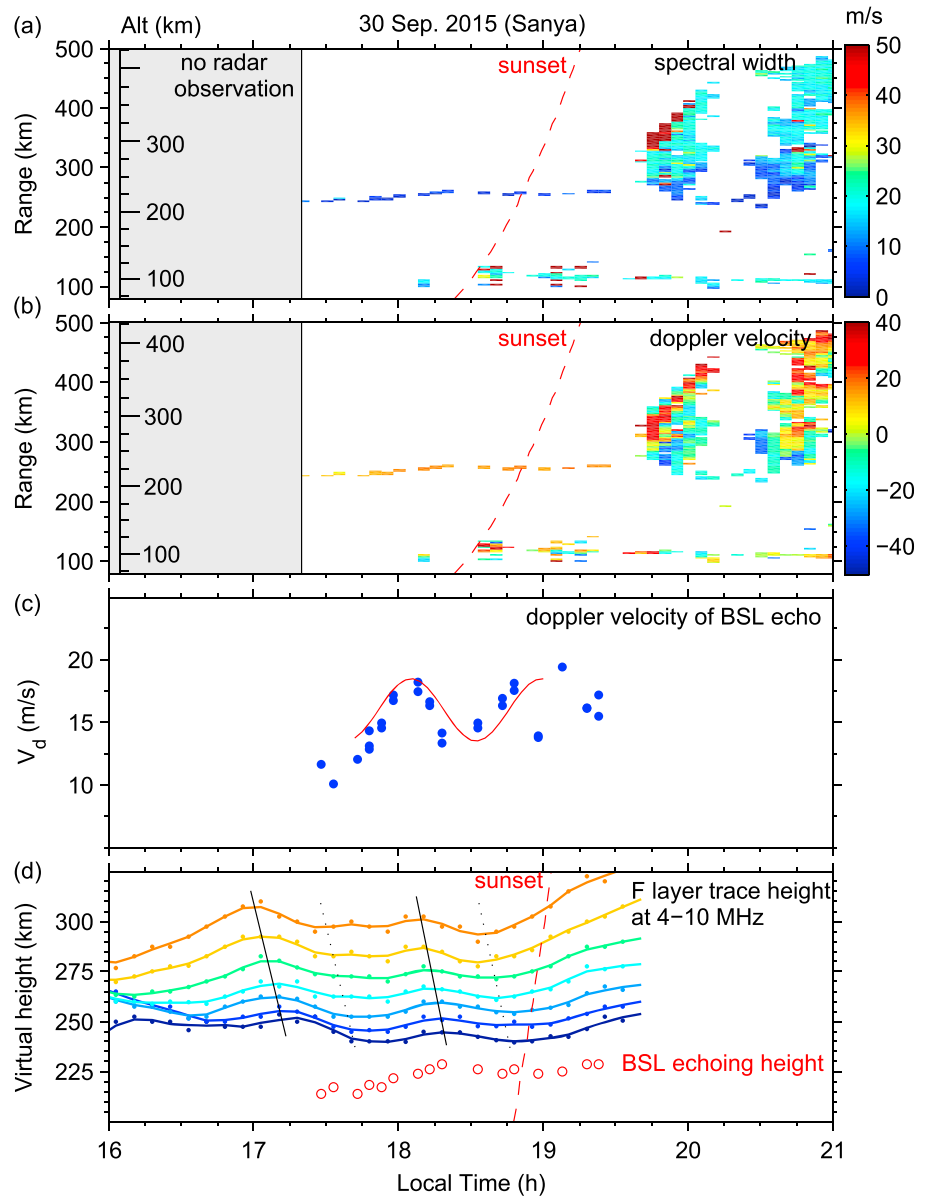
Figure 3. Range-time (a) Doppler spectral width and (b) Doppler velocity plots of irregularity echoes observed by the Sanya radar beam 3 (corresponding to Figure 2b) during 1720–2100 LT on 30 September 2015. The shaded area (gray) in the left of each panel indicates no F region observation. (c) Doppler velocities of BSL echoes. (d) F layer virtual heights (at seven plasma frequencies from 4 to 10 MHz) obtained from the Sanya ionograms. Small-amplitude oscillations can be seen in BSL echo Doppler velocity and F layer virtual heights.
