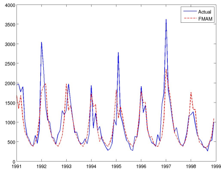
Figure 1. The streamflow prediction for the Furnas reservoir from 1991 to 1998.
