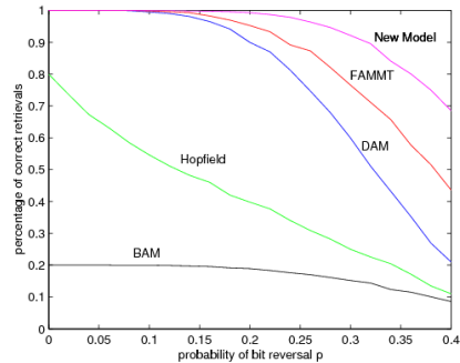
Figure 2. Percentage of Perfect Recall.
