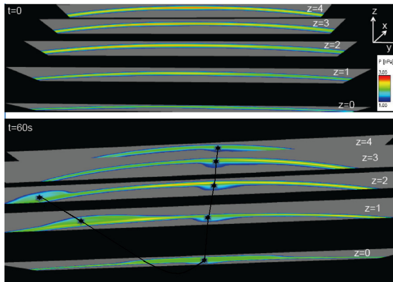
Fig. 10. Plasma pressure evolution for the z cuts ( z = 0, 1, 2, 3, 4 R_E ) at t = 0 (top image) and t = 60 s (bottom image). The observer sees the plots from bottom to top and anti-sunward.
