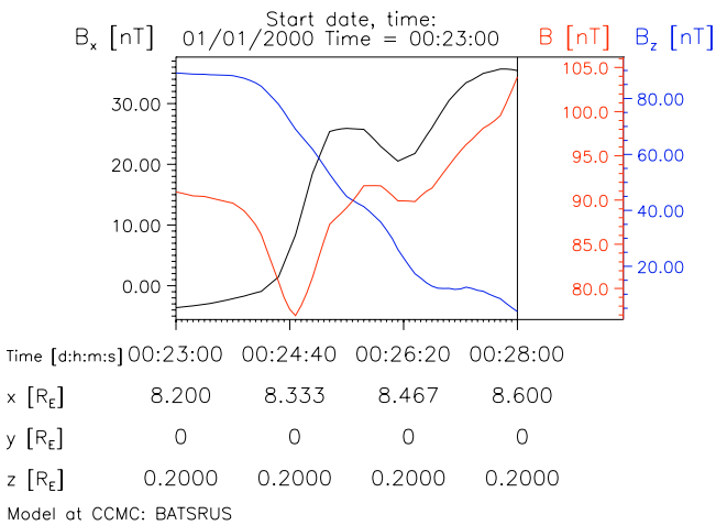
Fig. 5. Magnetic field data ( B_x , B_z , B ) from a virtual satellite crossing the northern part of the interlinked flux tubes. The satellite trajectory goes from the magnetosphere ( x = 8.2 R_E ) to the magnetosheath ( x = 8.6 R_E ) at y = 0 and z = 0.2 R_E . Red line refers to B , black to B_x and blue to B_z .
