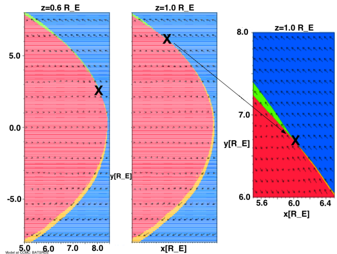
Fig. 13. Magnetic topology at t = 0 for positive z cuts at z = 0.6 and 1 R_E (first and middle plots), showing the X points. The third plot shows a zoom of the X point region at z = 1 R_E . Colors are related to magnetic topology as red, closed; yellow, connected to north; green, connected to south; and blue, solar wind. Arrows indicate flow velocity.
