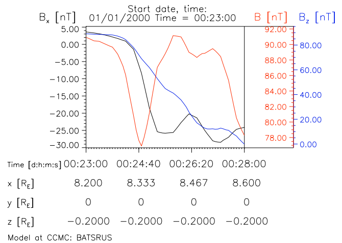
Fig. 6. Magnetic field data ( B_x , B_z , B ) from a virtual satellite crossing the southern part of the interlinked flux tubes. The satellite trajectory goes from the magnetosphere ( x = 8.2 R_E ) to the magnetosheath ( x = 8.6 R_E ) at y = 0 and z = -0.2 R_E .
