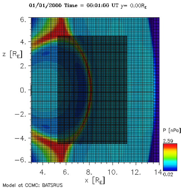
Fig. 1. Plasma pressure for the x - z plane at y = 0 at the beginning of the simulation. Earth is located at (0, 0, 0) . The finer resolution of 1/16 R_E is located around the magnetopause boundary layer. At this time the magnetopause subsolar point is located at x = 8 R_E and z = 0 .
