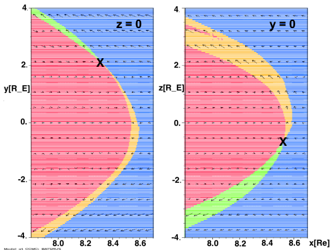
Fig. 17. Magnetic topology at t = 6 min 30 s for the noon-midnight plane ( z = 0 , first plot) and for the equatorial plane ( y = 0 , second plot). The X point is shifted from the subsolar point and located at z = -0.7 and y = 2.2 R_E . Colors are related to magnetic topology as red, closed; yellow, connected to north; green, connected to south; and blue, solar wind. Arrows indicate flow velocity.
