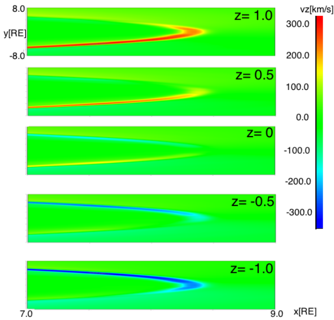
Fig. 3. Velocity in the z direction for z cuts ( z = +1, +0.5, 0, -0.5, -1 R_E ) on the x - y plane. The blue (red) region shows the flow direction roughly to south (north). The X line is located at the point of flow reversal.
