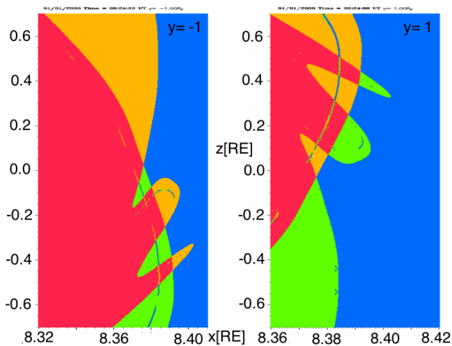
Fig. 15. Magnetic topology at t = 0 for y = -1 and 1 R_E . Colors are related to magnetic topology as red, closed; yellow, connected to north; green, connected to south; and blue, solar wind.
