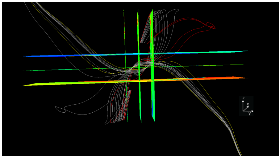
Fig. 11. Reconnected magnetic field lines drawn at t = 30 s. The lines exhibit the interlinked flux tubes configuration.
