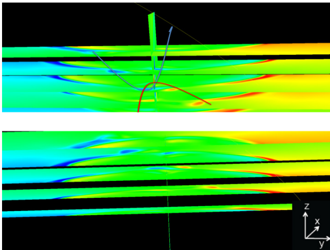
Fig. 12. Flow velocity in the y direction ( v_y ) for z cuts ( z = -2, -1, 0, 1, 2 R_E ) seen from two different perspectives: from above (top) and from below (bottom). Blue and red mean roughly downward and duskward flow, respectively. Red and blue lines have been drawn to indicate the flux tube shape.
