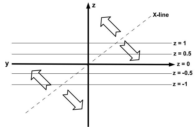
Fig. 2. Sketch of the magnetopause for the y - z plane. The tilted dashed line indicates the X line. The arrows represent the flow leaving the reconnection line. The lines at z = +1, +0.5, 0, -0.5, and -1 R_E indicate the z cuts shown in Fig. 3.
