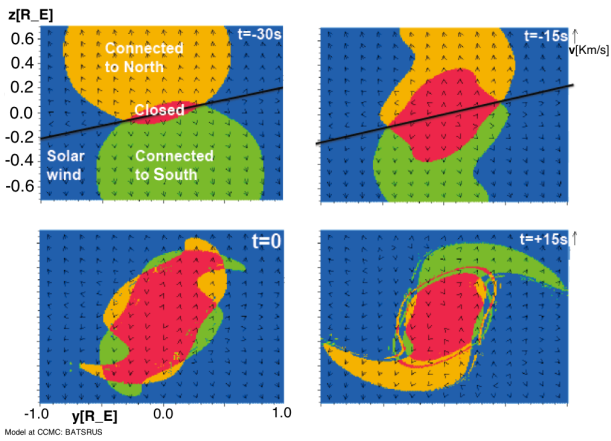
Fig. 8. Magnetic topology for the y - z plane at x = 8.41 R_E , looking anti-sunward, for different time instants: t = -30, -15, 0, +15 s, considering t = 0 as the time when the magnetic topology changes (interlinked flux tubes onset). Colors are related to the magnetic topology as red, closed; yellow, connected to north; green, connected to south; and blue, solar wind. Arrows indicate flow velocity. The black line indicates the single and tilted X line before the interlinked flux tubes onset.
