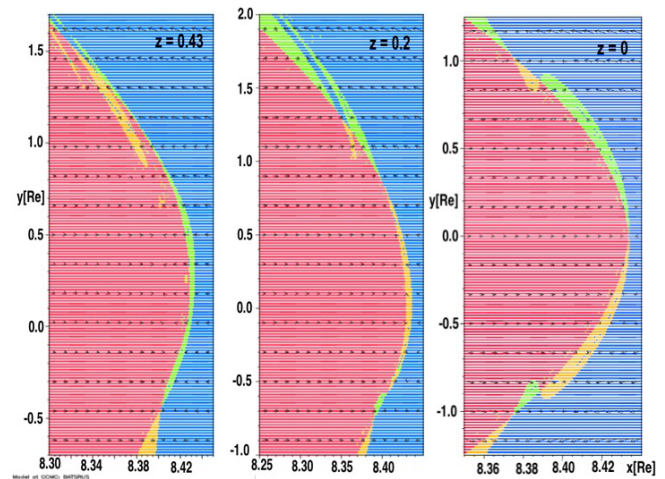
Fig. 14. Magnetic topology at t = 0 for z = 0.43, z = 0.2 and z = 0 R_E . Colors are related to magnetic topology as red, closed; yellow, connected to north; green, connected to south; and blue, solar wind. Arrows indicate flow velocity.
