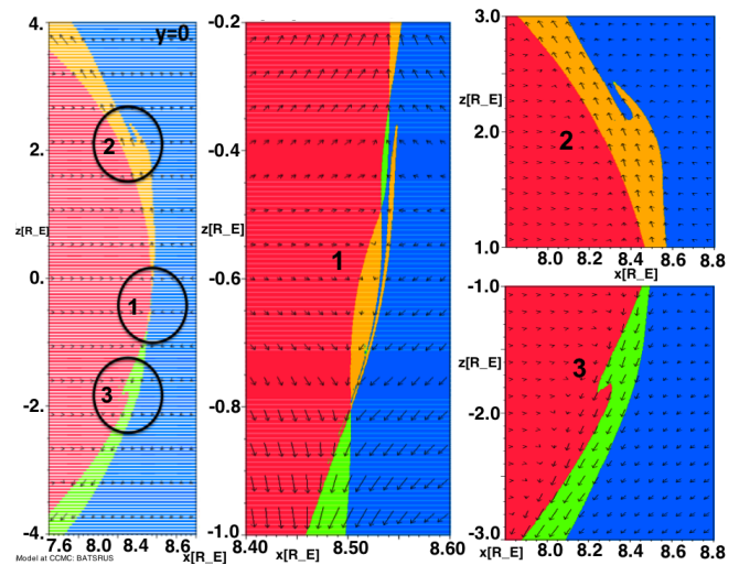
Fig. 18. Magnetic topology after the interlinked flux tubes had propagated northward, at t = 7 min, for the noon-midnight plane ( y = 0 , first plot), showing the numbered magnetic structures (1, 2, 3) displayed on a larger scale on the other three plots. Colors are related to magnetic topology as red, closed; yellow, connected to north; green, connected to south; and blue, solar wind. Arrows indicate flow velocity.
