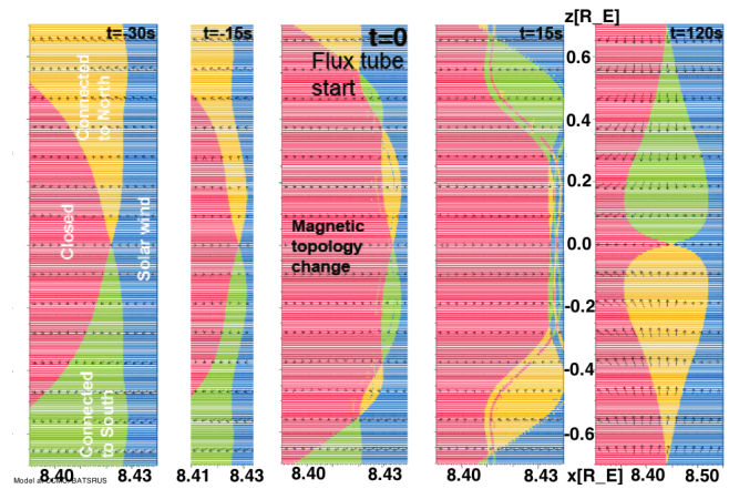
Fig. 9. Magnetic topology for the noon-midnight plane ( x - z plane) for different time instants: t = -30, -15, 0, +15, 120 s, considering t = 0 as the time when the magnetic topology changes (interlinked flux tubes onset). Colors are related to the magnetic topology as red, closed; yellow, connected to north; green, connected to south; and blue, solar wind. Arrows indicate flow velocity.
