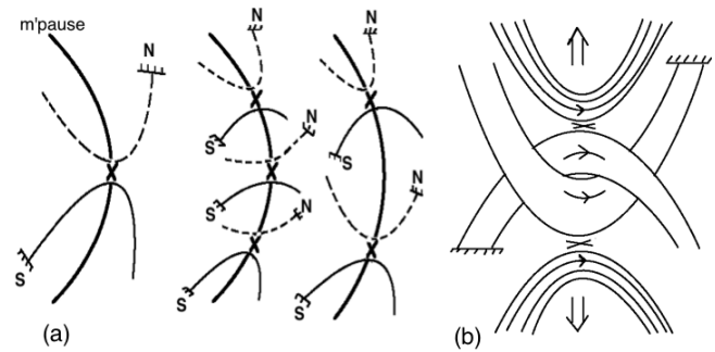
Fig. 4. (a) Sketch of the three steps in the X point configurations for the magnetic topology evolution in Fig. 9. The left panel in the sketch is the configuration for the topology shown at t = -30 and -15 s (first two panels in Fig. 9), the middle sketch refers to t = 0 (middle panel) and the sketch on the right to t = 15 and 120 s (two panels on the right). The m' pause line refers to the magnetopause and the X_s to the X points. The full and dashed lines are the reconnected magnetic field lines coming out from the reconnection site, and connected to Earth's Southern (S) and Northern (N) Hemispheres. (b) Sketch illustrating the structure of two interlinked flux tubes. We show magnetic field lines and tubes on the magnetopause seen from the Sun. The X_s indicate the two possible reconnection sites responsible for such magnetic field configuration.
