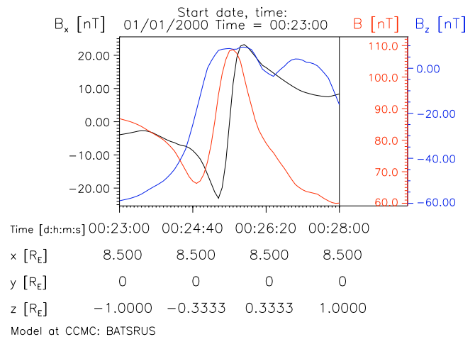
Fig. 7. Magnetic field data ( B_x , B_z , B ) from a virtual satellite crossing the interlinked flux tubes in the z direction. The satellite trajectory goes from z = -1 to 1 R_E at x = 8.5 R_E and y = 0 .
