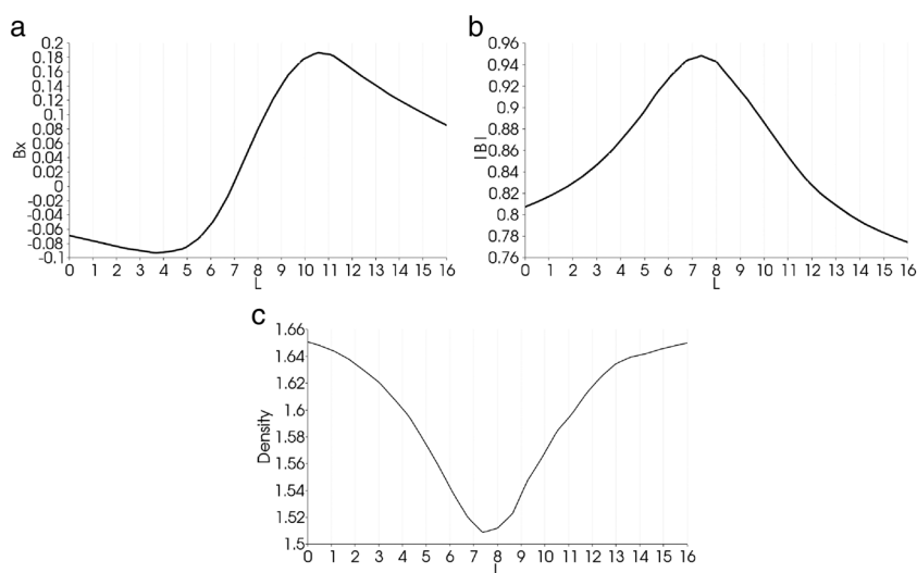
Figure 9. Plots of the component of the magnetic field normal to (top, left) the magnetopause, (top, right) the total field strength, and (bottom) plasma density for trajectory T4. This trajectory have a length of 16L_0 ( \approx 6400 km) along the z direction, parallel to the magnetopause, going from z = 17L_0 to z = 33L_0 , and is located at x = 5L_0 ( \approx 2000 km) from the center of the magnetopause into the magnetosheath. The x axis corresponds to the length of the trajectory starting from z = 17L_0 . All plots are presented in normalized units.
