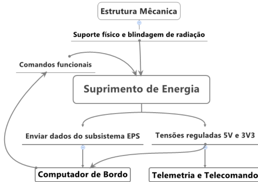
Figura 28 – Diagrama de interface do subsistema EPS.
