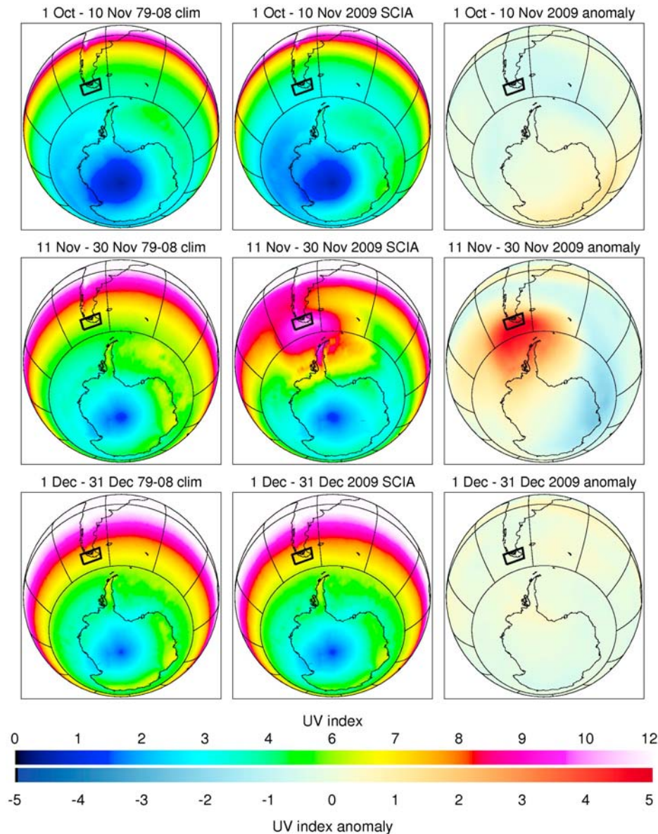
Figure 2. As Figure 1 but for UVI values. 1 UVI unit equals 25 mW/m 2 .
