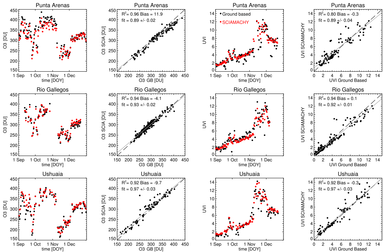
Figure 4. Time series for 2009 of ground-based and satellite measurements of total O 3 columns (first column; in DU) and ground-based UVI measurements as well as satellite total O 3 column based UVI values (third column) and the corresponding scatter plots (second and fourth column) for the three locations on the southern tip of South America, summarized in Table 1. The fit values in the scatter plots are calculated for an ordinary linear regression.
