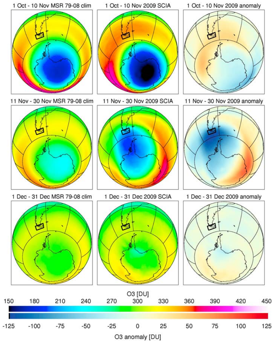
Figure 1. Average total O 3 columns for the periods (top) 1 October – 10 November, (middle) 11–30 November and (bottom) 1–31 December for the (left) 1979–2008 MSR total O 3 column climatology, (middle) the assimilated SCIAMACHY total O 3 columns for 2009 and (right) the 2009 total O 3 column anomaly with respect to the MSR total O 3 column climatology. Total O 3 column values and anomalies are in Dobson Units ( \sim 2.69 \cdot 10^{16} molecules/cm 2 ). The box area around the most southern tip of South America represents the area used for Figure 3.
