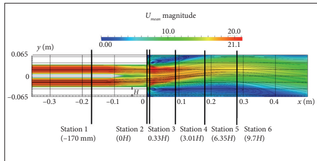
Figure 6. Mean velocity field, streamlines and stations in case i2 /configuration 3.
