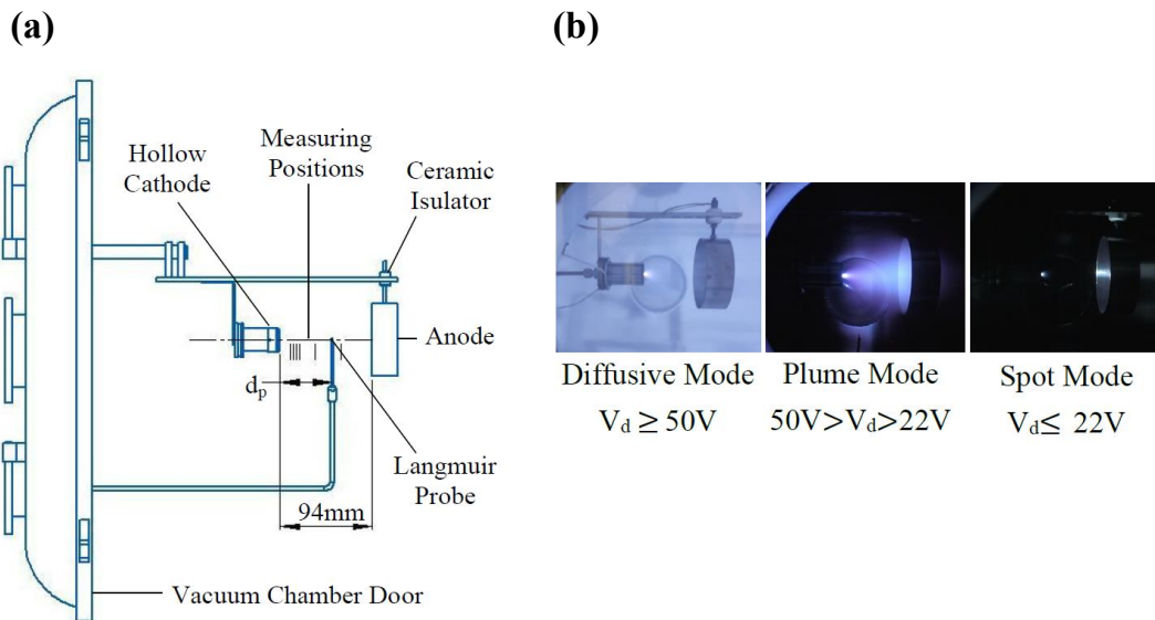
Figure 1. Experimental setup (a) and discharge modes of hollow cathodes (b).
