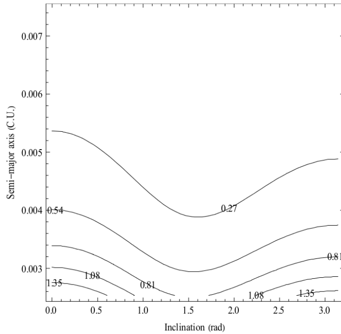
Figure 4. PI_1 as a function of the semi-major axis (in canonical units) and inclination (in radians) of circular orbits for the spacecraft considering the third-body effects of Jupiter, the terms coming from the rotating frame and the irregular shape of Europa.
