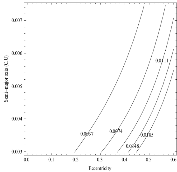
Figure 13. PI_3 as a function of the semi-major axis (in canonical units) and eccentricity for eccentric orbits for spacecraft considering the effects of the irregular shape of Europa.
