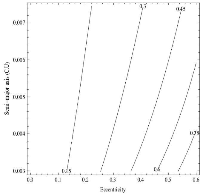
Figure 12. PI_3 as a function of the semi-major axis (in canonical units) and eccentricity for eccentric orbits for spacecraft considering the effects of the irregular shape of Europa, the third-body perturbation from Jupiter and the effects of the rotating frame.
