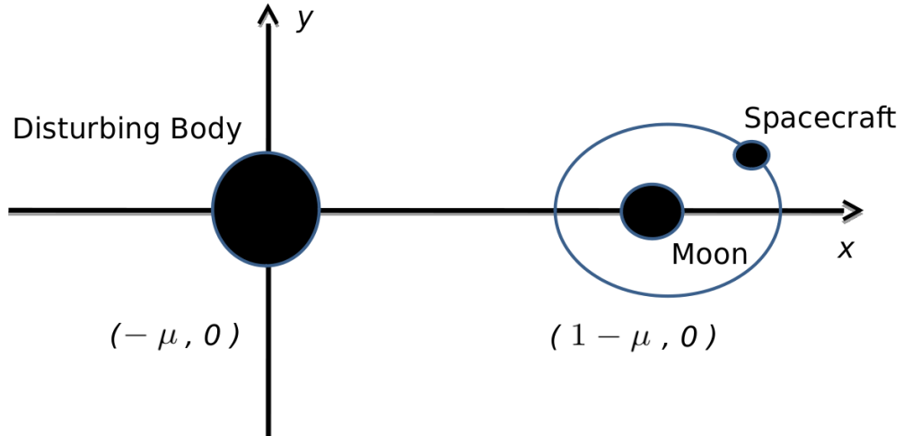
Figure 1. Geometry of the Restricted Three Body Problem.
