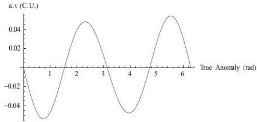
Figure 5. PI_2 for an Europa orbiter
