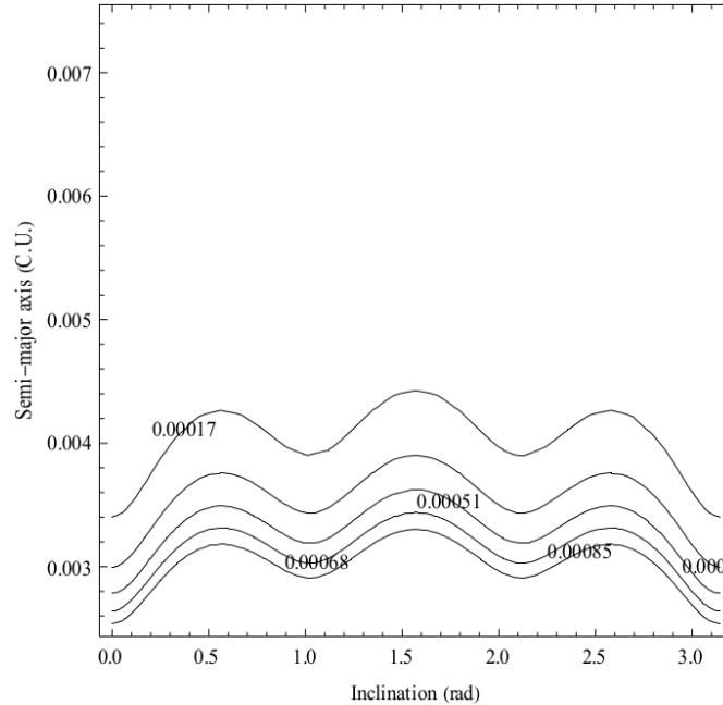
Figure 2. PI_1 as a function of the semi-major axis (in canonical units) and inclination (in radians) of circular orbits for the spacecraft considering only the effects of the irregular shape of Europa.
