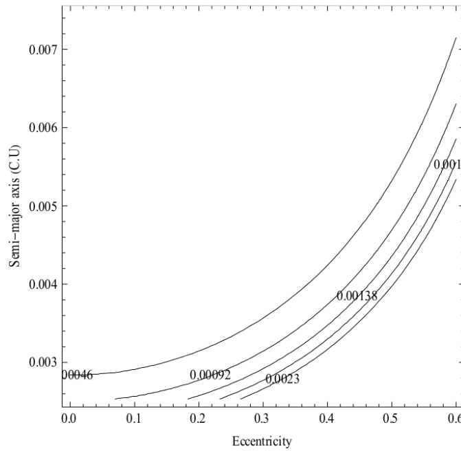
Figure 10. PI_1 as a function of the semi-major axis (in canonical units) and eccentricity for eccentric orbits for spacecraft considering the effects of the irregular shape of Europa.
