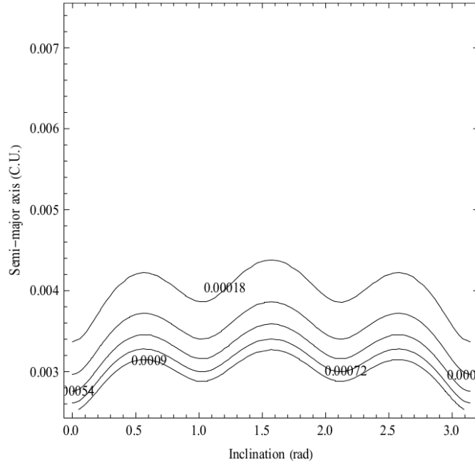
Figure 6. PI_1 as a function of the semi-major axis (in canonical units) and inclination (in radians) for eccentric orbits for spacecraft considering the effects of the irregular shape of Europa.
