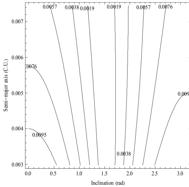
Figure 9. PI_3 as a function of the semi-major axis (in canonical units) and inclination (in radians) for eccentric orbits for spacecraft considering the effects of the third-body perturbation from Jupiter and the effects of the rotating frame.
