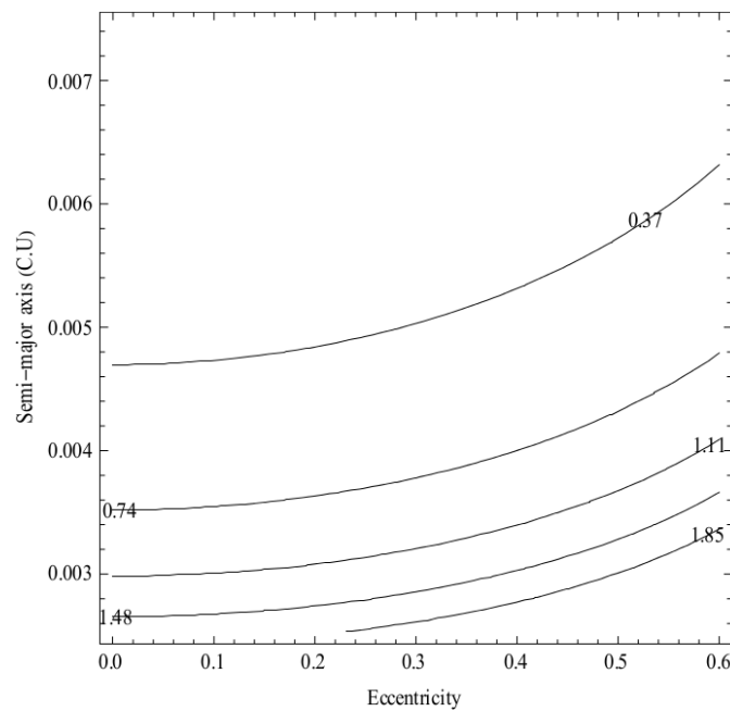
Figure 11. PI_1 as a function of the semi-major axis (in canonical units) and eccentricity for eccentric orbits for spacecraft considering the effects of the irregular shape of Europa, the third-body perturbation from Jupiter and the effects of rotating frame.
