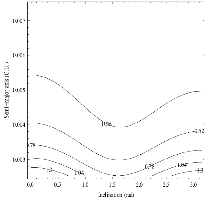
Figure 3. PI_1 as a function of the semi-major axis (in canonical units) and inclination (in radians) of circular orbits for the spacecraft considering only the third-body effects of Jupiter and the terms coming from the rotating frame.
