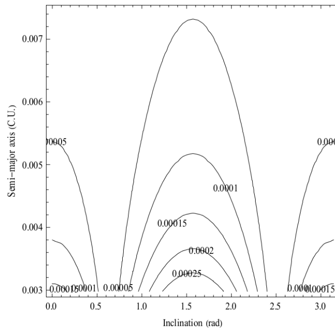
Figure 8. PI_3 as a function of the semi-major axis (in canonical units) and inclination (in radians) for eccentric orbits for spacecraft considering the effects of the irregular shape of Europa.
