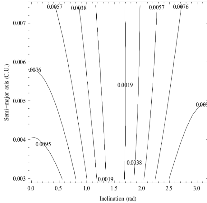
Figure 7. PI_3 as a function of the semi-major axis (in canonical units) and inclination (in radians) for eccentric orbits for spacecraft considering the third-body effects of Jupiter, the irregular shape of Europa and the terms due to the rotating frame.
