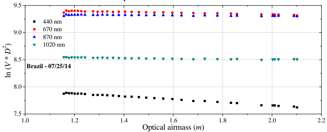
Figure 4.6. Langley graph on July 25 th , 2014 in Brazil site, for spectral bands of the CE317/CIMEL sun photometer.
