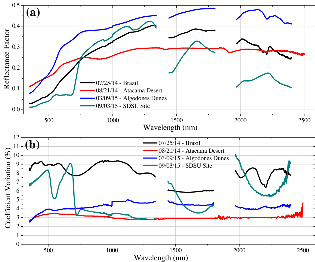
Figure 4.5. In (a) Spectral reflectance results of the reference sites; and (b) surface coefficient of variation in percentage.
