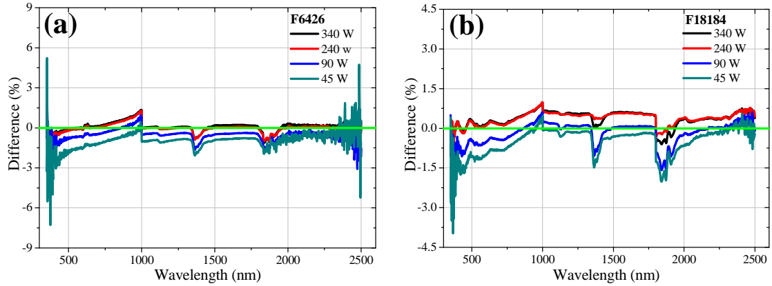
Figure 4.2. Difference between the measurements with the integrating sphere source made before and after fieldwork as a function of the wavelength. In (a) with the FieldSpec F6426; and (b) with the FieldSpec F18184. The differences presented in this figure are from laboratory 1 compared with laboratory 2. The results during laboratory 3 were similar.
