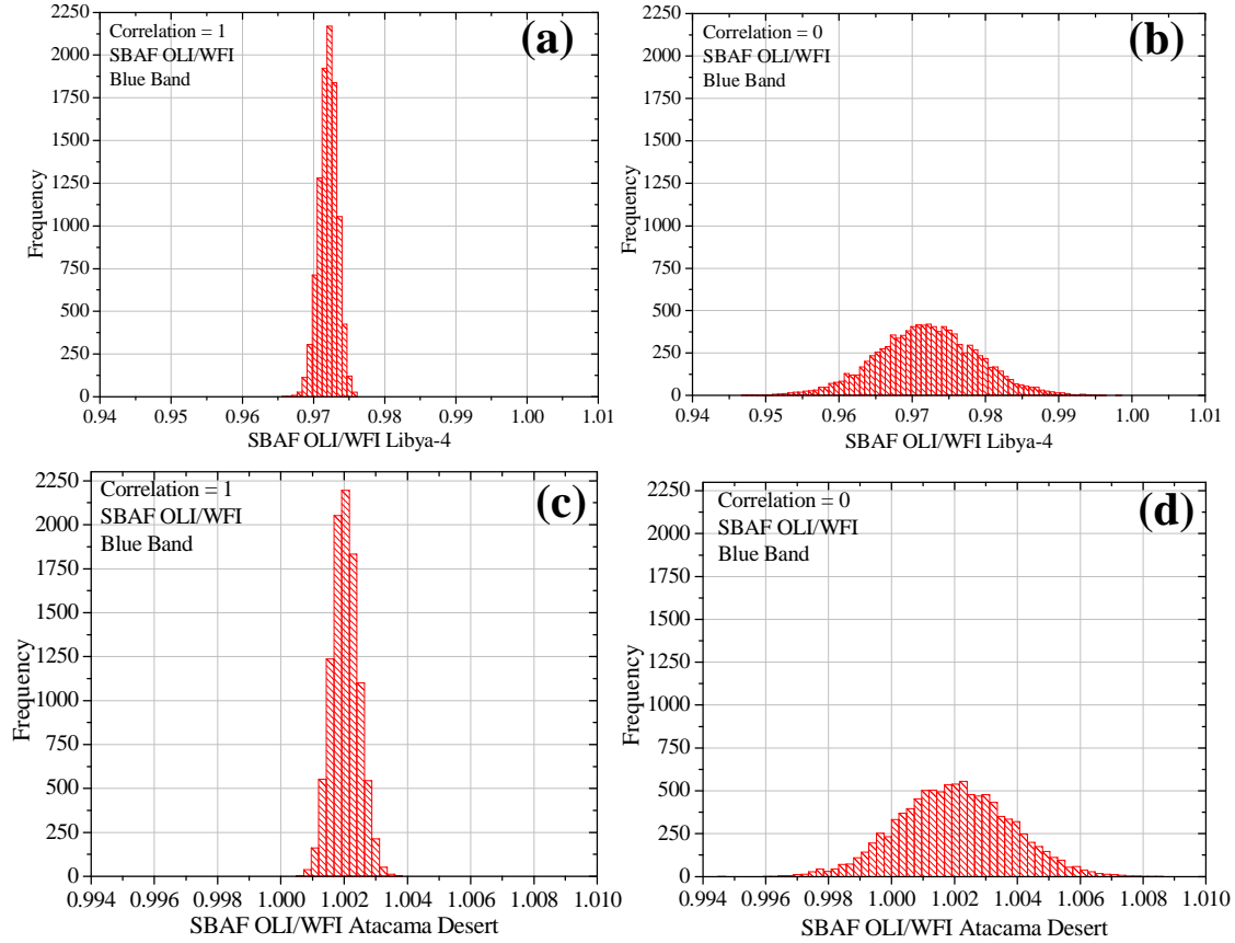
Figure 4.16. Simulated SBAF histogram used to compensate the WFI/CBERS-4 TOA reflectance to match OLI/Landsat-8 TOA reflectance. In (a) Libya-4 site with maximum correlation; (b) Libya-4 site with minimum correlation; (c) Atacama Desert site with maximum correlation; (d) Atacama Desert site with minimum correlation.
