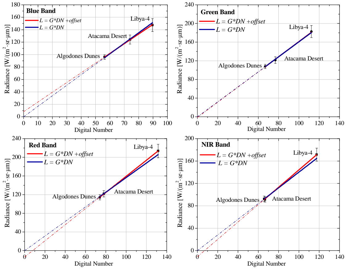
Figure 4.17. Radiometric calibration of MUX/CBERS-4.
