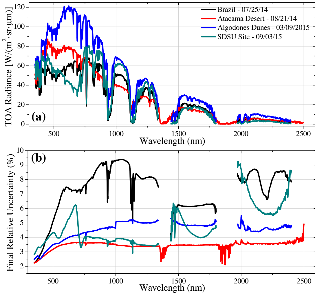
Figure 4.12. In (a) TOA radiance predicted by MODTRAN; and (b) its final relative uncertainty (in percentage).
