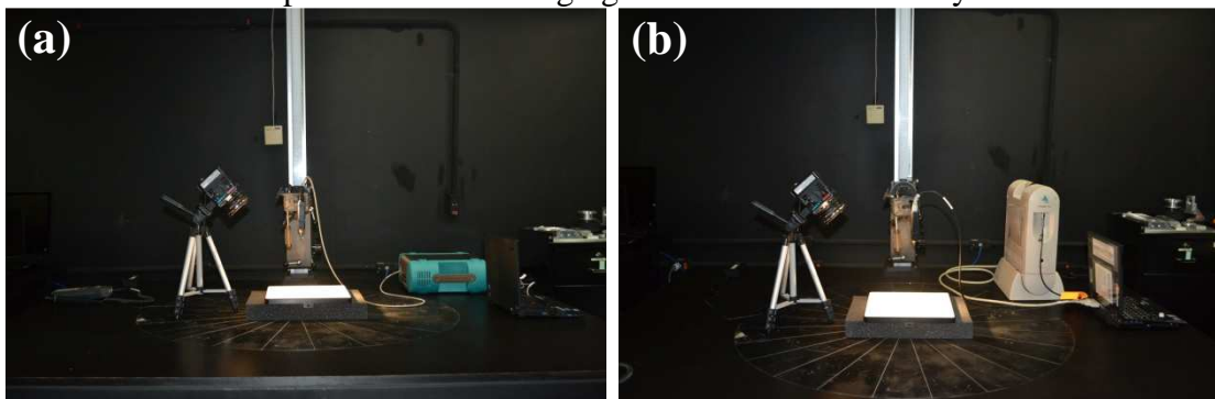
Figure 3.10. Overview of the experimental setup to characterize and assess the reference panel used in fieldwork. In (a) measurements with the FieldSpec Pro ASD used in fieldwork; and (b) measurements with the FieldSpec Pro ASD belonging to the LaRaC laboratory.
