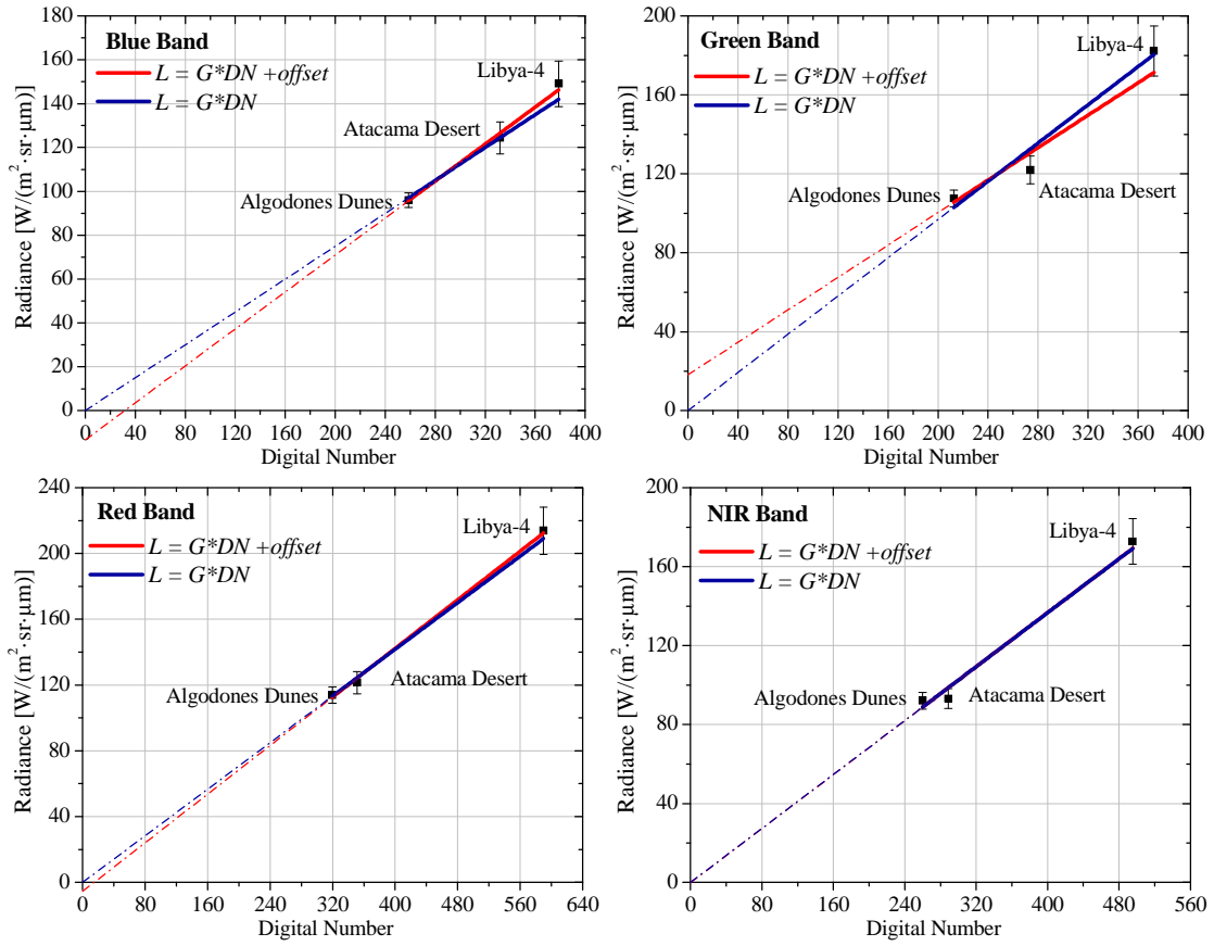
Figure 4.18. Radiometric calibration of WFI/CBERS-4.
