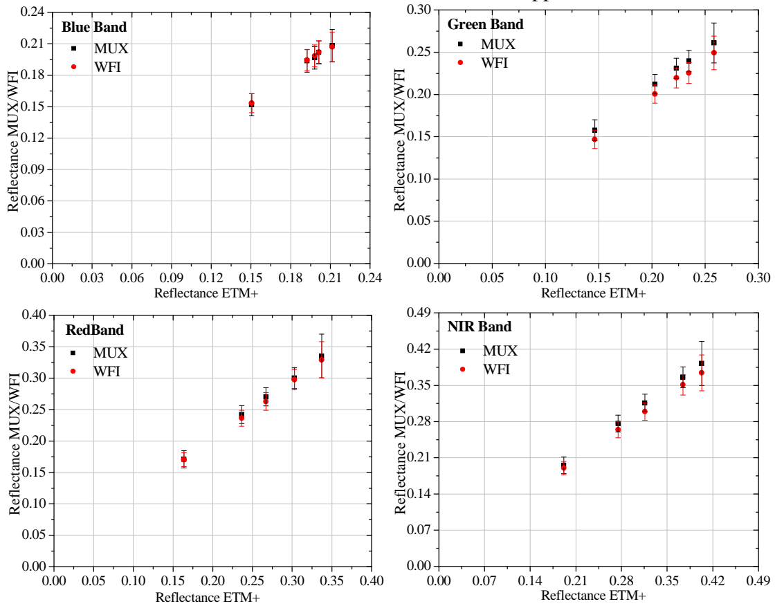
Figure 4.21. TOA reflectance comparison between ETM+/Landsat-7 and MUX/CBERS-4 and WFI/CBERS-4 after application of the SBAF.
