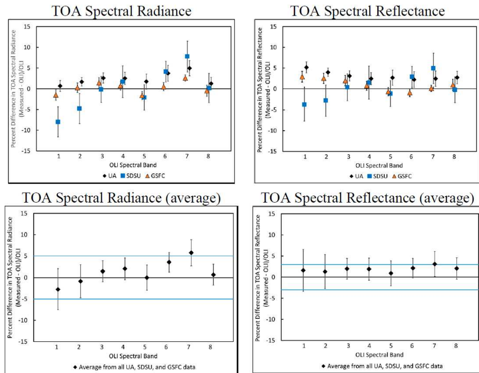
Figure 3.2. A summary of in situ results from the University of Arizona (UA), South Dakota State University (SDSU), and Goddard Space Flight Center (GSFC) for TOA spectral radiance (top left) and reflectance (top right) for OLI/Landsat-8. The uncertainty bars are the 1\sigma standard deviation of the measurements by each team. Note that band 9 (cirrus) is excluded from the results due to an extremely low Signal-to-Noise Ratio (SNR) in the ground measurements. The bottom row shows the results for TOA spectral radiance (bottom left) and reflectance (bottom right) when the ground-based results from all three teams are consolidated into one data set and then compared to OLI/Landsat-8. The uncertainty bars in the average graphs are the 1\sigma standard deviation of the average from all three teams.
