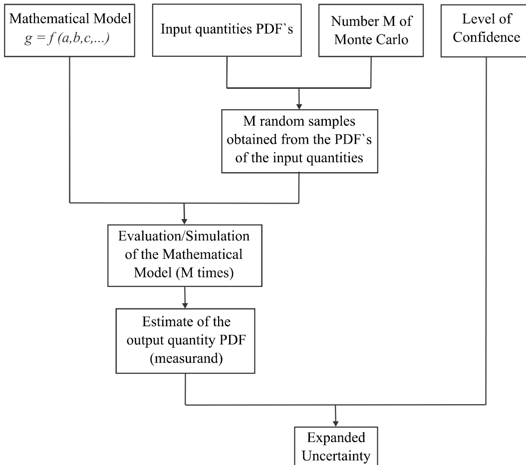
Figure 2.5. The propagation and summarizing stages of uncertainty evaluation using Monte Carlo method to implement the propagation of distributions.
