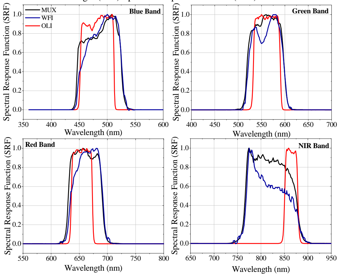
Figure 2.3. Multispectral Camera (MUX), Wide-Field Imager (WFI) and Operational Land Imager (OLI) Spectral Response Function (SRF).
