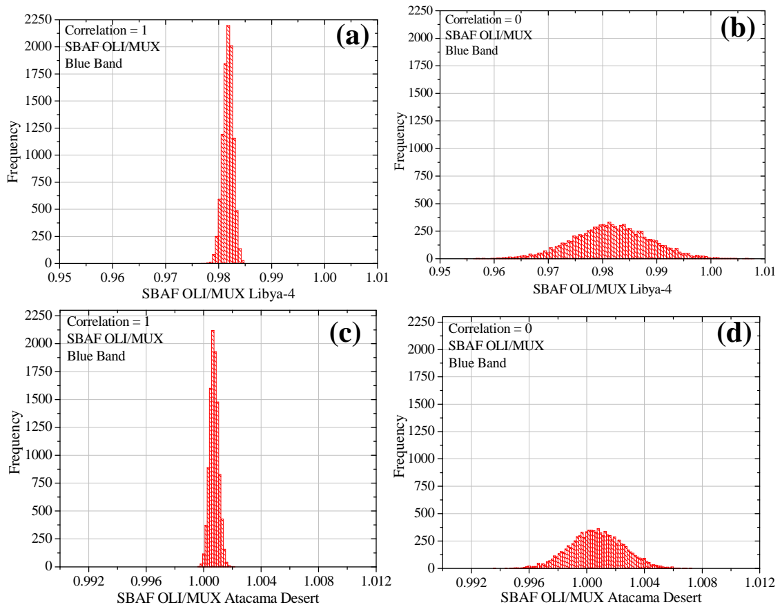
Figure 4.15. Simulated SBAF histogram used to compensate the MUX/CBERS-4 TOA reflectance to match OLI/Landsat-8 TOA reflectance. In (a) Libya-4 site with maximum correlation; (b) Libya-4 site with minimum correlation; (c) Atacama Desert site with maximum correlation; (d) Atacama Desert site with minimum correlation.
