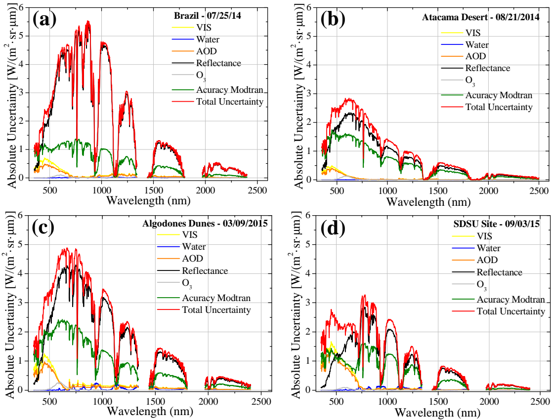
Figure 4.11. TOA radiance uncertainty predicted by MODTRAN. In (a) on July 25 th , 2014 in Brazil site; (b) on August 21 st 2014 in Atacama Desert, Chile; (c) on March 9 th 2015 in Algodones Dunes, USA; and (d) on September 3 th 2015 in SDSU site.
