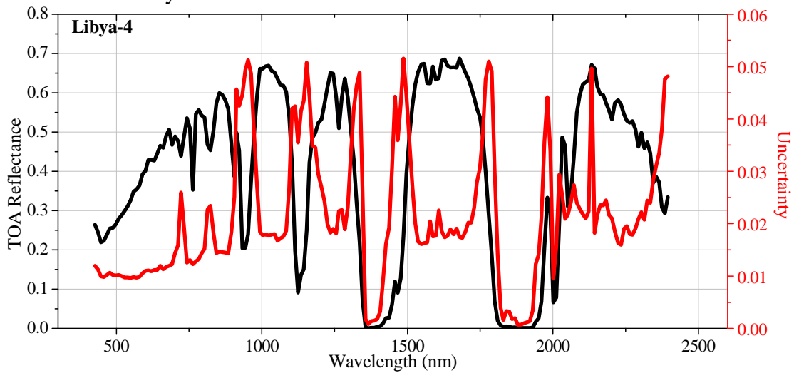
Figure 3.22. Average TOA reflectance profile of 224 Hyperion/EO-1 images over Libya-4 from 2004 to 2014.
