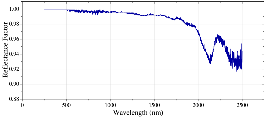
Figure 3.9. Spectral reflectance of the standard panel from LaRaC.
