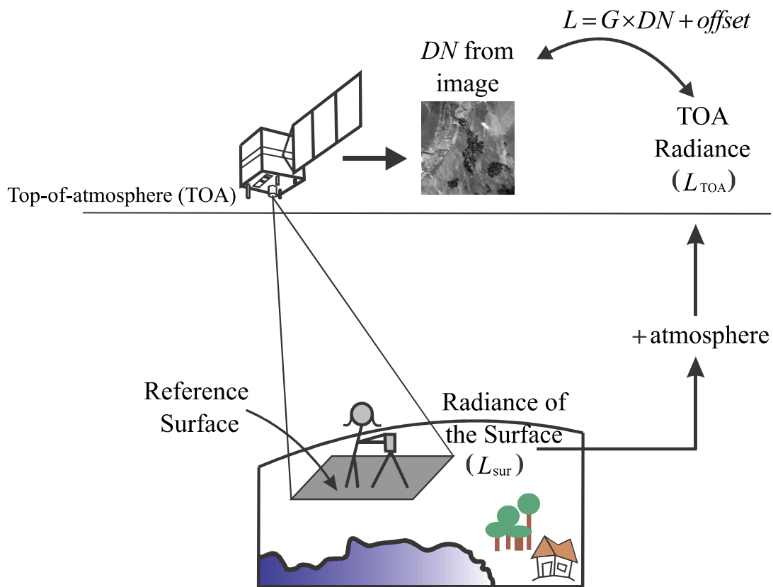
Figure 2.1. Illustrative scheme of reflectance-based approach procedures.
