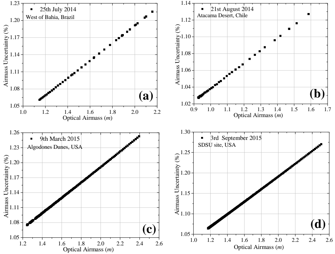
Figure 3.15. Optical airmass uncertainties. In (a) on 25 July 2014 in Brazil; (b) on 21 August 2014 in Atacama Desert; (c) on 9 March 2015 in Algodones Dunes; (d) on 3 September 2015 in SDSU site.
