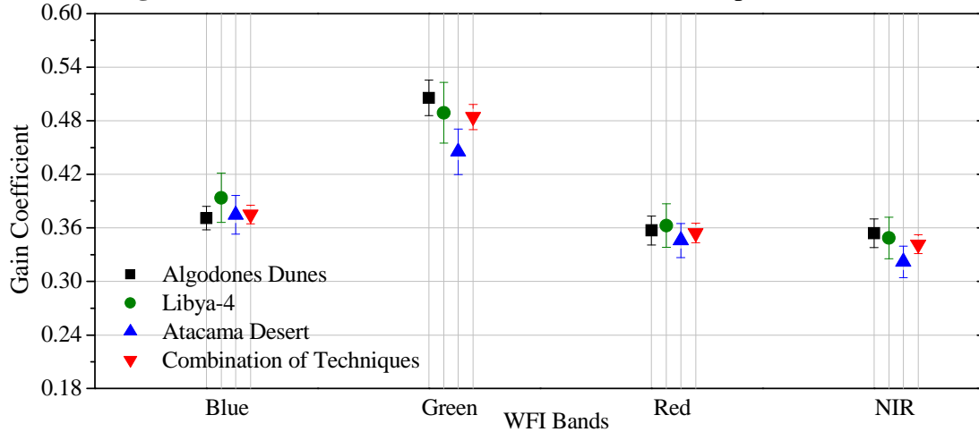
Figure 4.20. Gain coefficients of the WFI/CBERS-4 spectral bands.
