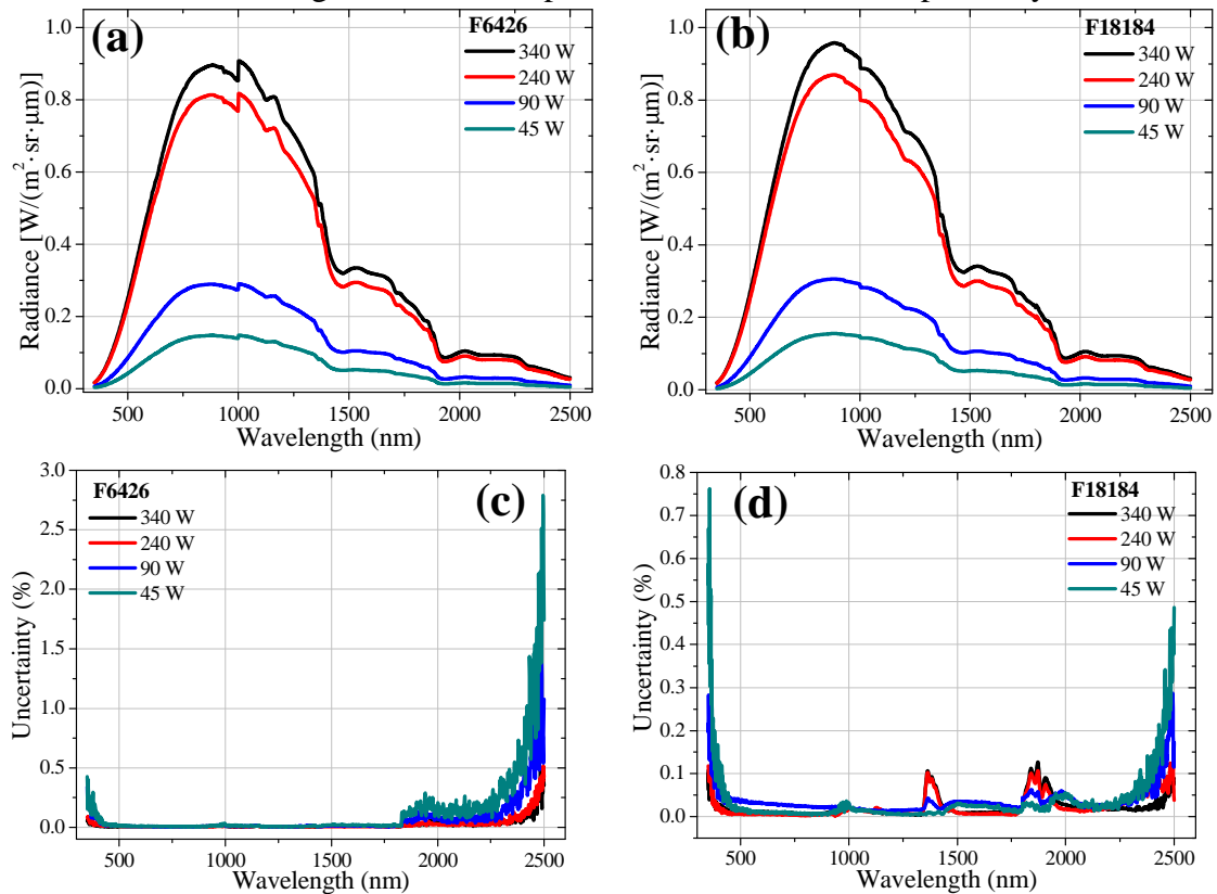
Figure 4.1. In (a) and (b) radiance as a function of wavelength of the FieldSpec F6426 and F18184, respectively; and (c) and (d) relative uncertainty as a function of wavelength of the FieldSpec F6426 and F18184, respectively.
