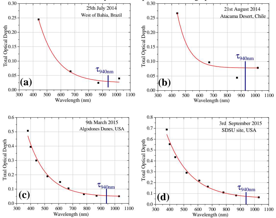
Figure 3.16. Total Optical depth at 940 nm. In (a) on 25th July 2014 in Brazil; (b) on 21th August 2014 in Atacama Desert; (c) on 9th March 2015 in Algodones Dunes; (d) on 3rd September 2015 in SDSU site. The uncertainties are very small comparable with the graph scale.
