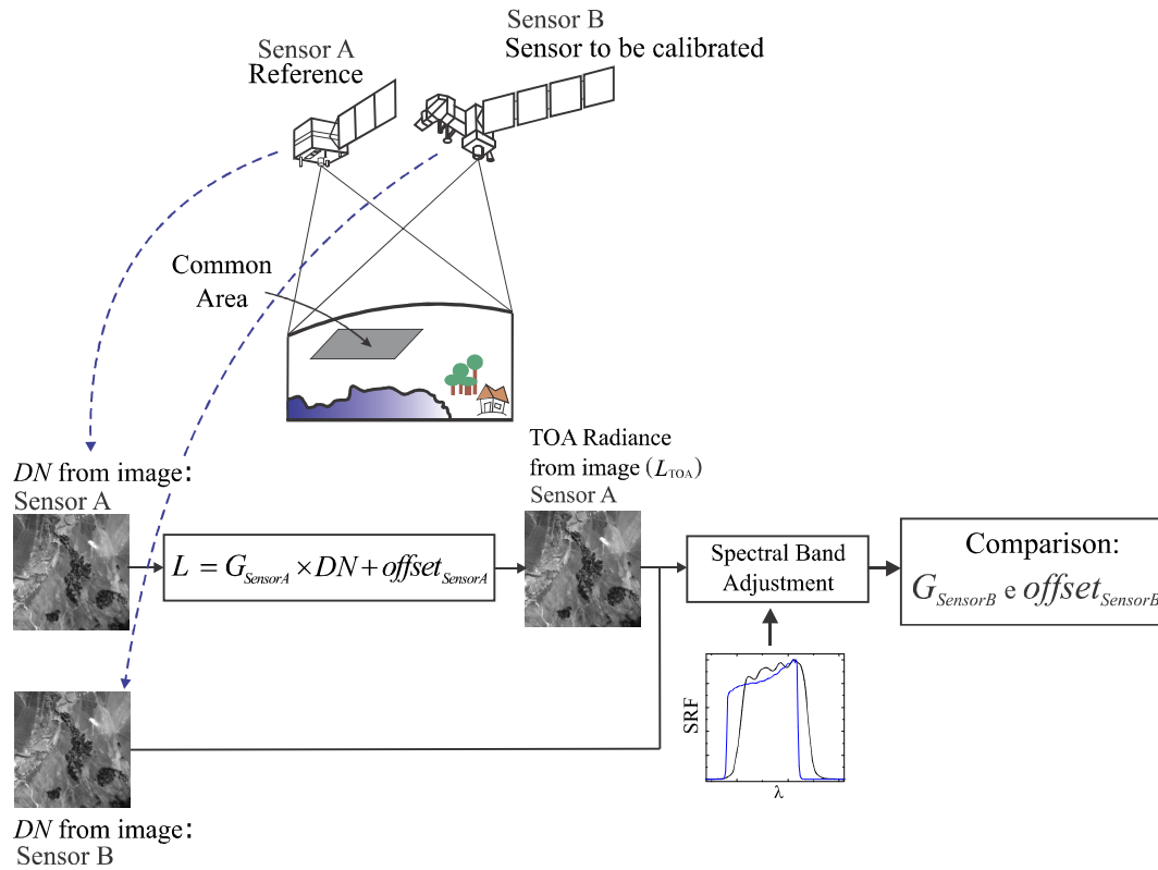
Figure 2.2. Illustrative scheme of cross-calibration method procedures.
