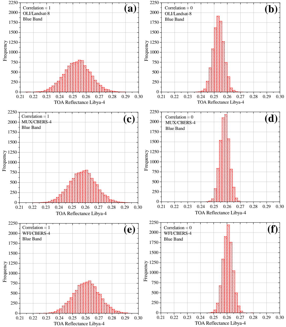
Figure 4.14. Simulated reflectance factor histogram for the spectral blue band and for Libya-4 site. In (a) and (b) sensor OLI/Landsat-8 with maximum and minimum correlation, respectively; (c) and (d) sensor MUX/CBERS-4 with maximum and minimum correlation, respectively; (e) and (f) sensor WFI/CBERS-4 with maximum and minimum correlation, respectively.
