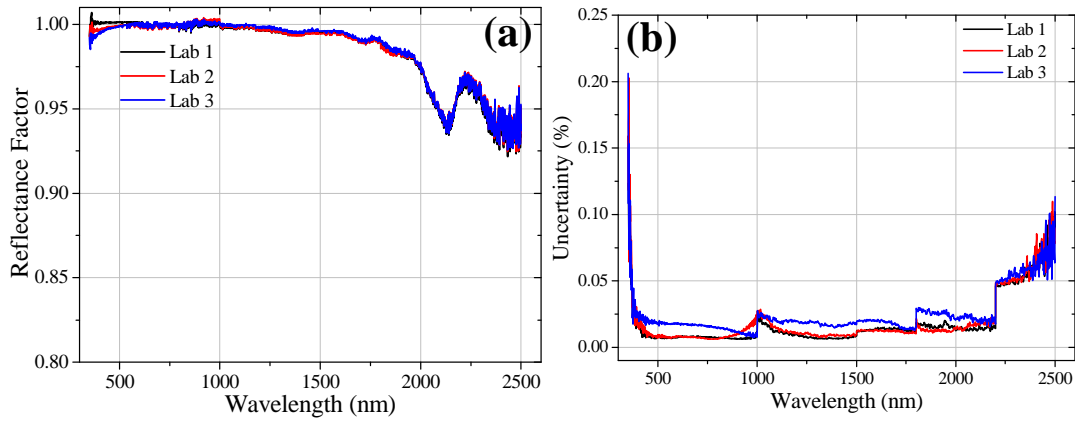
Figure 4.3. In (a) reflectance factor of the panel reflectance used in fieldwork as a function of wavelength; and (b) uncertainties (mean standard deviation) as a function of wavelength.
