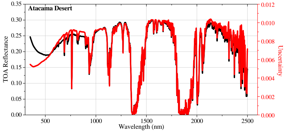
Figure 3.23. Average TOA reflectance over Atacama Desert profile from ground measurements.
