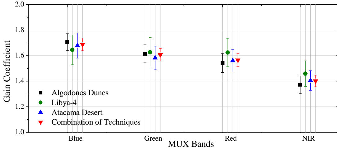
Figure 4.19. Gain coefficients of the MUX/CBERS-4 spectral bands.
