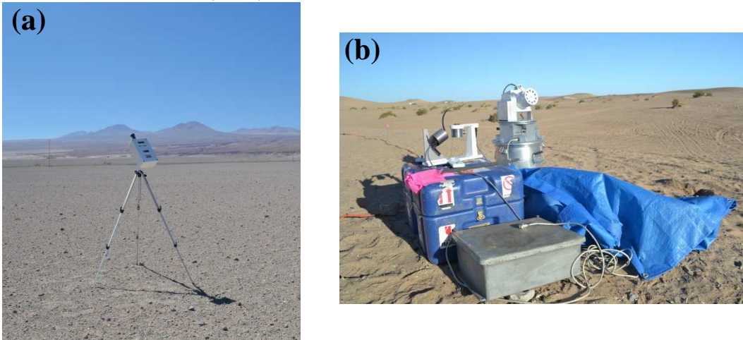
Figure 3.12. In (a) the sun photometer CE317/CIMEL; and (b) Automated Solar Radiometer (ASR).
