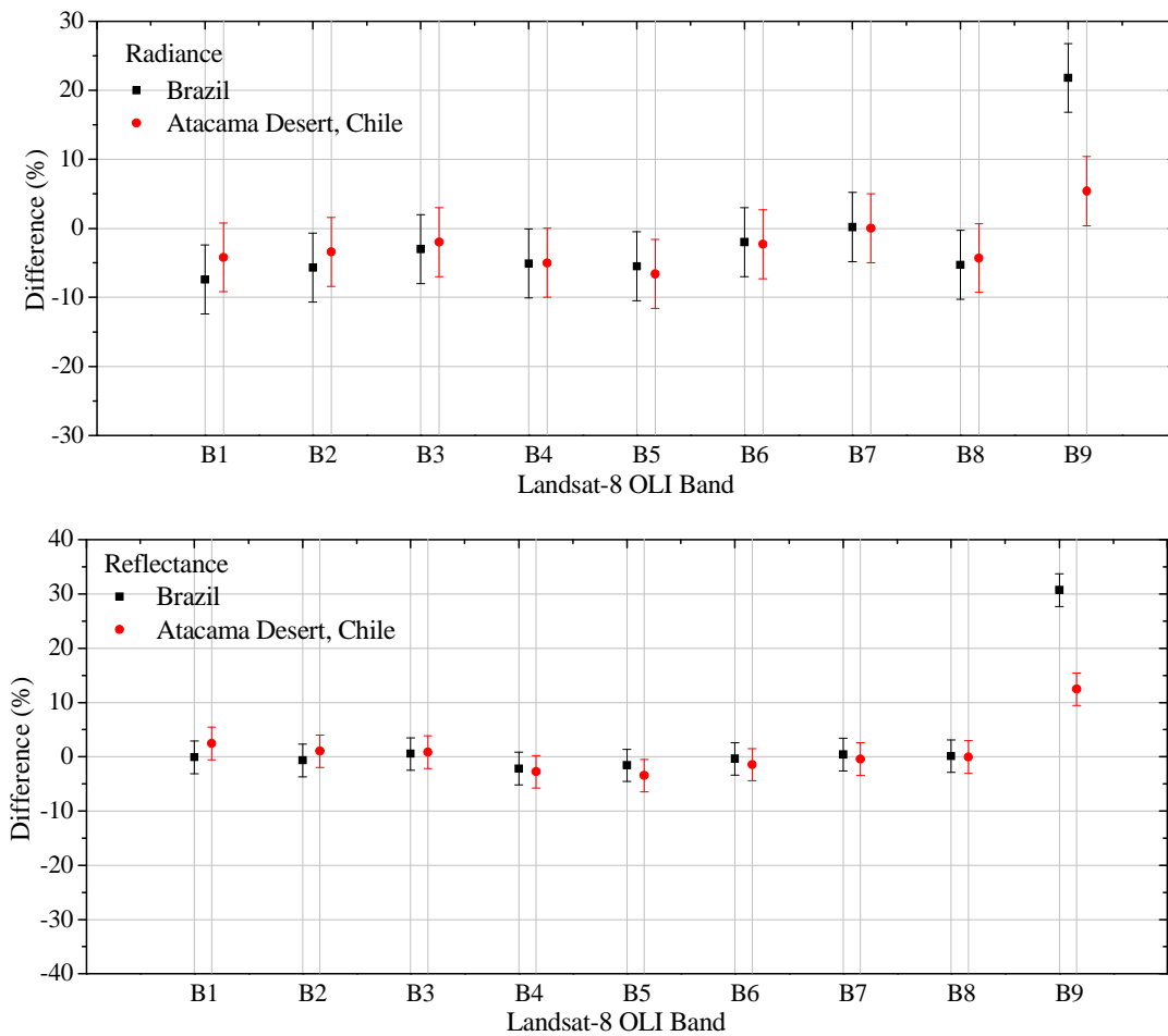
Figure 4.13. Comparison of radiance/reflectance reported by OLI/Landsat-8 and radiance/reflectance predicted with the reflectance-based approach. The error bars in this graph are the uncertainties of OLI/andsat-8 sensor (5% in radiance and 3% in reflectance).
