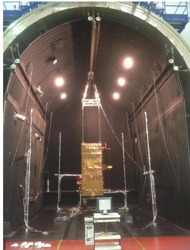
Fig. 4 - TM loaded into the LIT-INPE 6m x 8m Space Simulation Chamber
