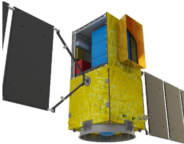
Fig. 1 - The Amazonia-1 Satellite
