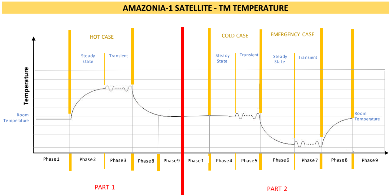
Fig. 6 - Amazonia-1 Thermal Model Thermal-Vacuum Test Profile
