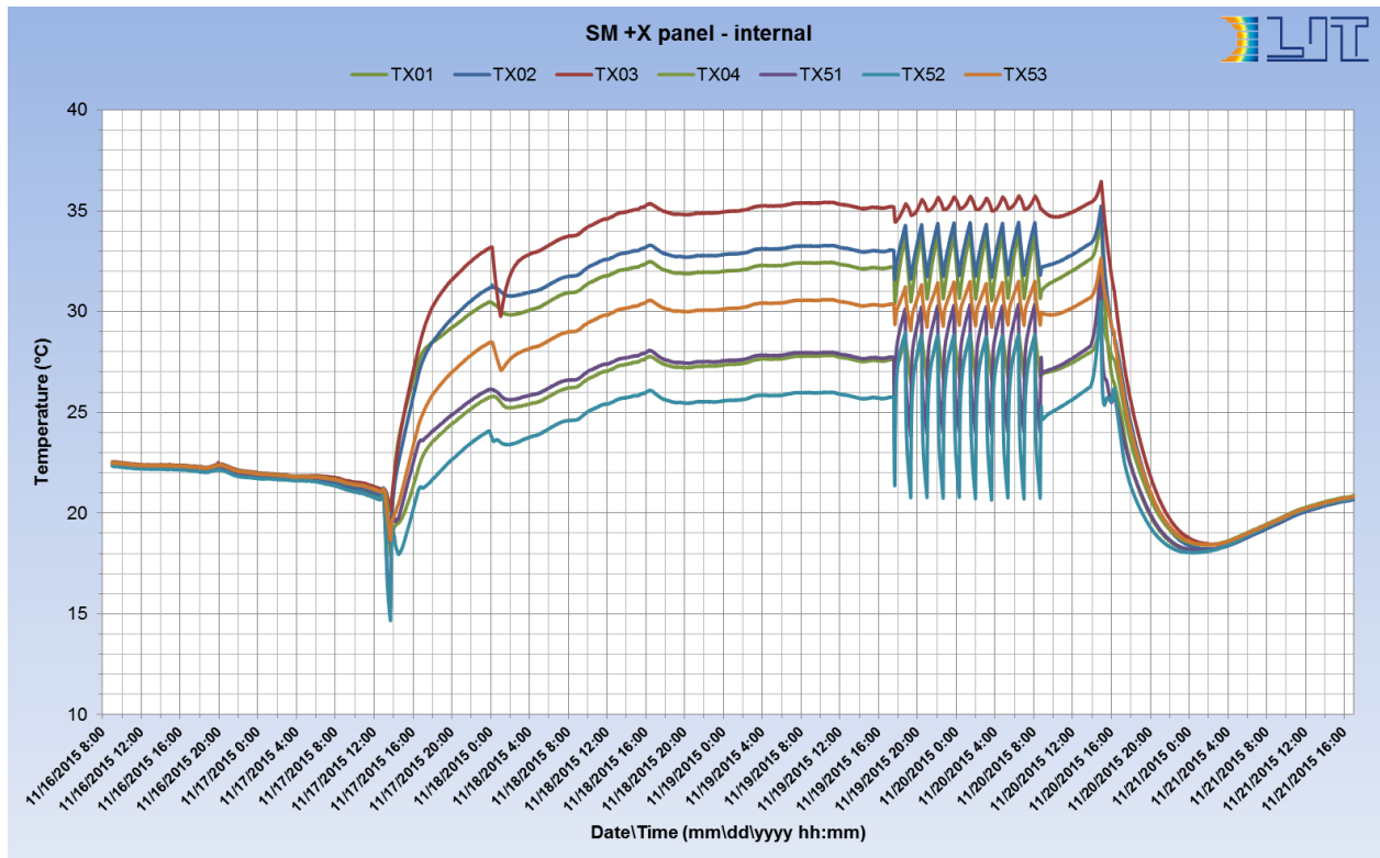
Fig. 7 - Example of Temperature Development at an S/C Section During the TBT
