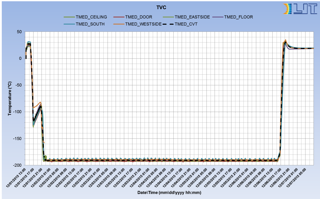
Fig. 8 - Temperature on the TVC Thermal Shrouds - part 2 of TBT
