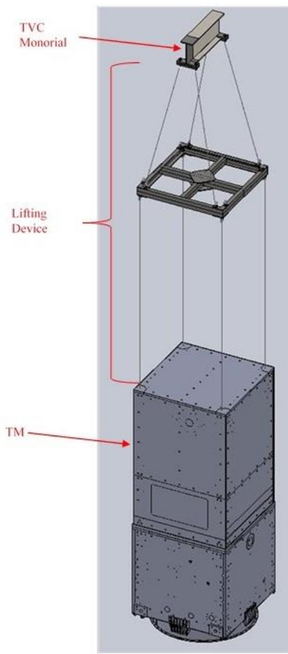
Fig. 3 - Spacecraft lifting device
