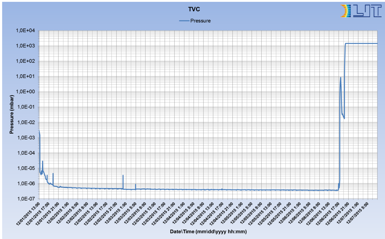
Fig. 9 - Vacuum Level on the TVC - part 2 of TBT
