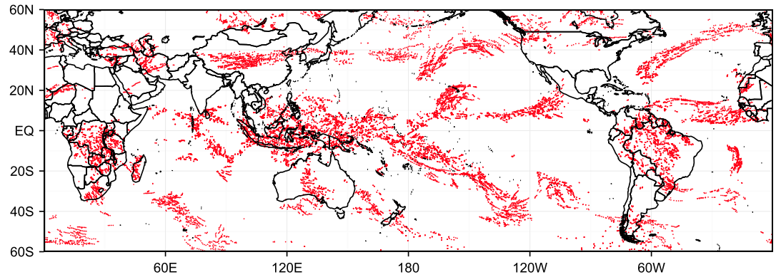
Figure 3. Cloud cluster tracks from 1–4 December 2001 produced from using the ForTrACC algorithm. A few days of tracking yield a large number of clusters, and their movement begins to trace out large-scale atmospheric patterns.
