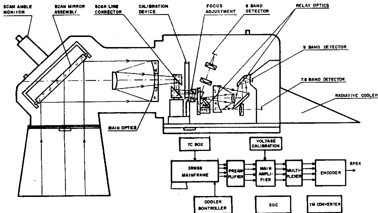
Figure 4: IR Multispectral Scanner
