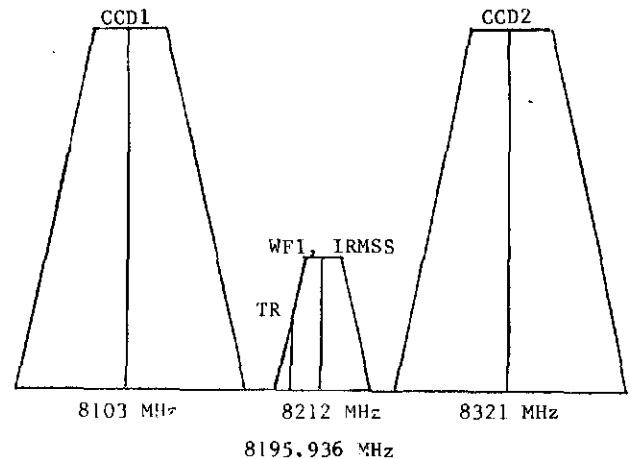
Figure 6: RF Spectrum
