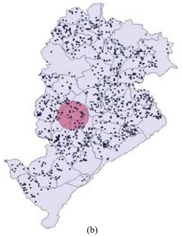
Fig. 1 - (a) Number of mosquito eggs gathered from an egg trap in Recife, Brazil; and (b) Occurrences of meningitis in Belo Horizonte city.
