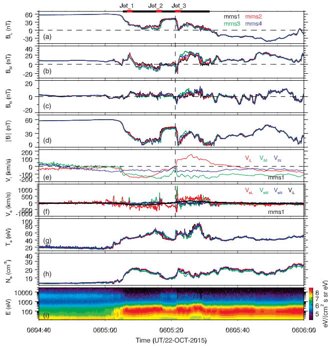
FIG. 1. (a)–(d) B_L , B_M , B_N , and |\mathbf{B}| at the four satellites, (e) ion flows v_{iL} , v_{iM} , and v_{iN} , and (f) electron flows v_{eL} , v_{eM} , v_{eN} , and v_{eI} at mms1. The electron (g) temperature, (h) density, and (i) energy spectrum at mms1.
