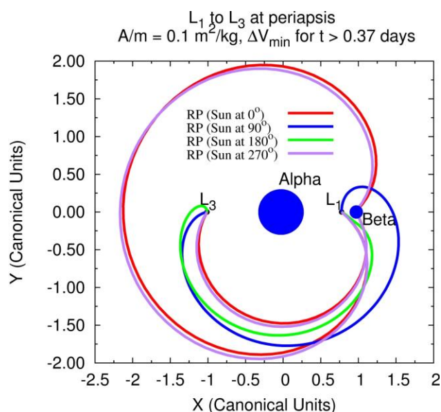
Figure 1. Trajectories between the Lagrange points of the asteroid 1996FG 3 considering the radiation pressure.
