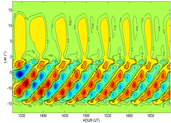
Figure 2: Meridional neutral wind perturbation run obtained by taking the difference in the integrated electron density at current time from initial time.
