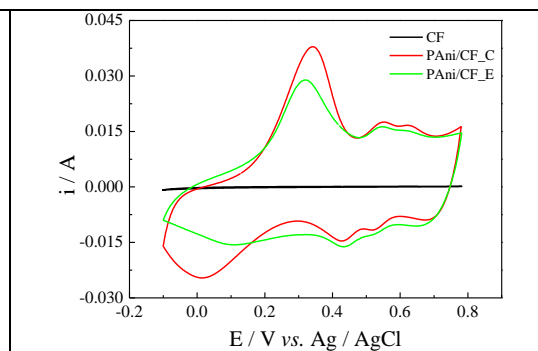
Fig. 2. CV curves of PANi/CF obtained by both methods at a scan rate 25 mV s -1 .
