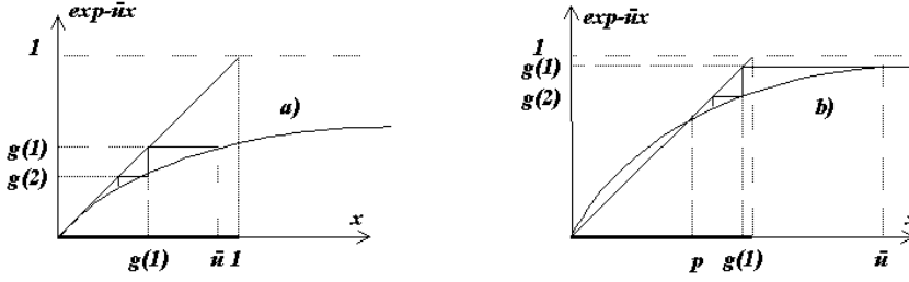
Figure 4. (a) The weight \bar{u} < 1 , then g(n) \rightarrow 0 , as n \rightarrow \infty . (b) The weight \bar{u} \geq 1 , then g(n) \rightarrow p , as n \rightarrow \infty .
