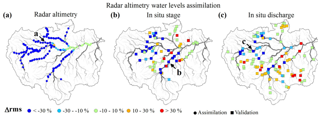
Fig. 4. Evaluation of ENVISAT radar altimetry data assimilation. Spatial distribution of change in root-mean-square error ( \Delta_{\text{rms}} ) at (a) altimetry stations used for data assimilation and stream gauges with (b) stage and (c) discharge data used for verification.
