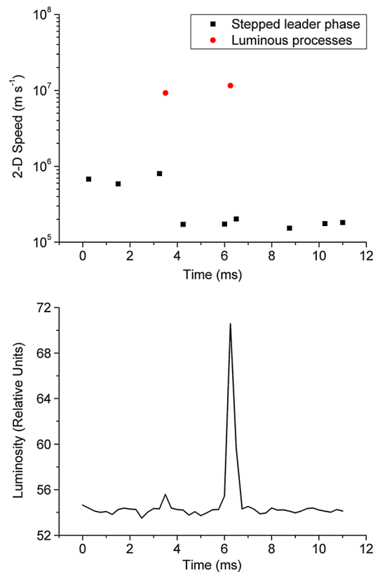
Figure 3. Temporal evolution of the (top) 2-D leader partial speed and (bottom) luminosity computed during the \beta_2 leader in Case 1. Time t=0 corresponds to the frame in which the leader first became visible in the camera field-of-view, and the return stroke occurred at t=13.75 ms. SL stands for the stepped leader phase and LP for luminous process. The first LP ( t=3.50 ms) could have only its minimum speed estimated.
