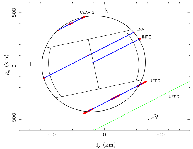
Figure 3. The best elliptical fit to the occultation chords for the event of 2010 using the times from Table 1 and the pole-constrained solution. The arrow indicates the direction of motion, blue lines are the observed chords, the red segments are the ingress, egress and mid-occultation error bars at 1\sigma level.
