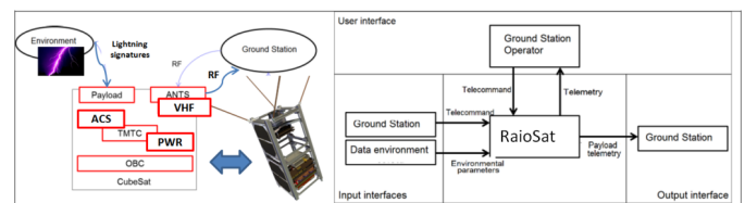
Fig. 8. RaioSat architecture (physical / interface diagram)
