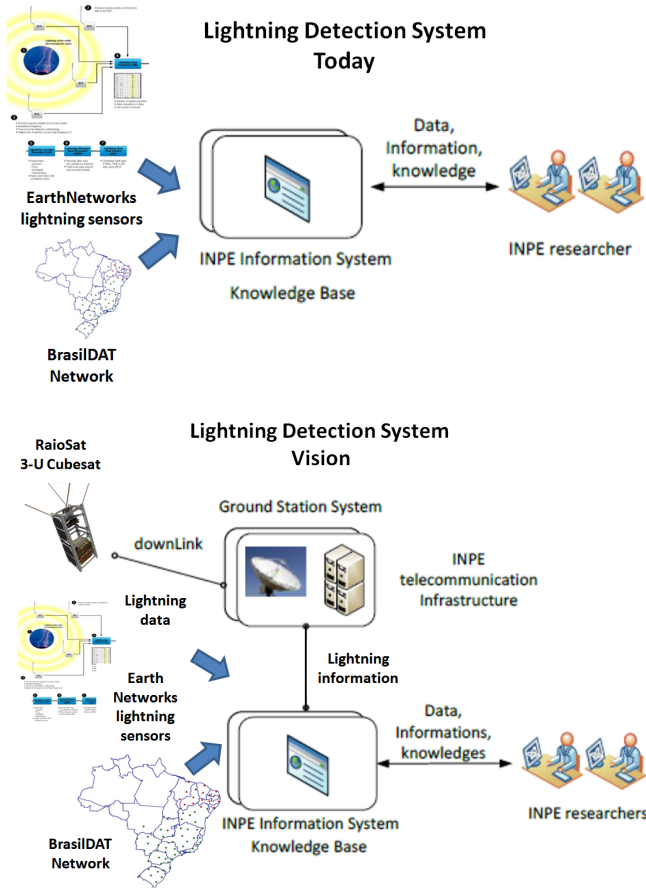
Fig. 4. Operation Concept of the Lightning Detection System.
