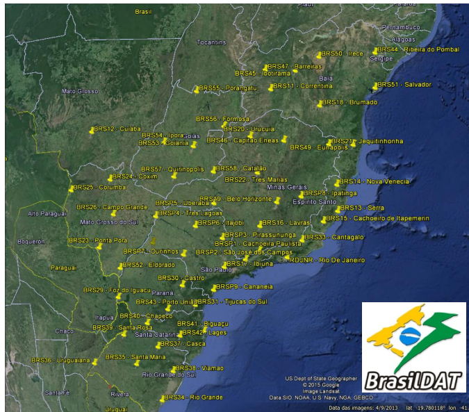
Fig. 1. Present sensor configuration of the BrasilDAT total lightning detection system with 56 installed sensors.
