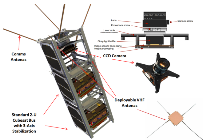
Fig. 9. Preliminary structure and payload elements for the RaioSat system.
