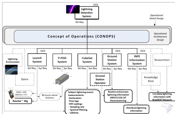
Fig. 5. Concept of Operation (ConOps) of the Lightning Detection System
