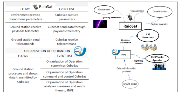
Fig. 6. RaioSat event list with essential function and context diagram
