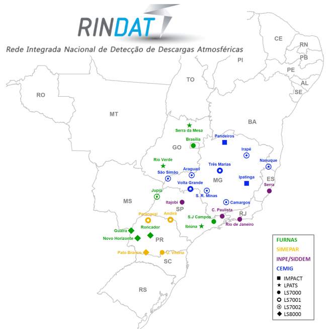
Fig. 2. Present sensor configuration of the RINDAT lightning detection system with 27 installed sensors.
