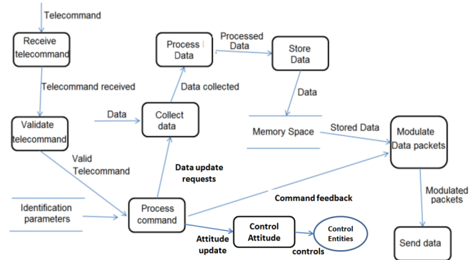
Fig. 7. RaioSat event list with essential function and context diagram
