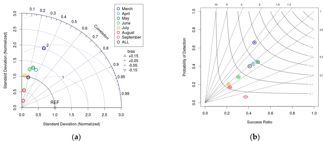
Figure 3. Taylor diagram (a) and performance diagram (b) showing monthly metrics of IMERG (satellite) versus S-band SIPAM radar (reference) from March–September 2014. Color dots indicate different months. On the Taylor diagram, angular axes show COR, whereas radial axes show IMERG SD (the centered RMS difference (solid gray line)) normalized against the reference. The triangle symbol and its direction (up/down) indicate the percent bias (positive/negative). On the performance diagram, dashed lines represent bias scores with labels on the outward extension of the line, while labeled solid contours correspond to critical success index (CSI); the x- and y-axis represent the success ratio (SR) and POD, respectively; and sampling uncertainty is given by the crosshairs.
