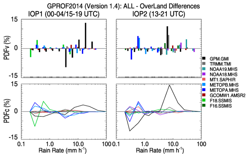
Figure 10. Differences between the original PDFv (top) and PDFc (bottom) distributions and the overland only GPROF2014 rainfall retrievals over the Manaus region during IOP1 (during 00–04 UTC and 15–19 UTC, left) and IOP2 (during 13–21 UTC, right). Each bar and each line represent the contribution of precipitation over inland water (along the Negro, Solimões and Amazon rivers) for all sensor measurements used in the GPROF2014 algorithm.
