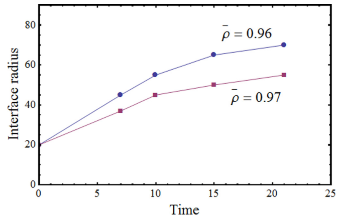
FIG. 4. Radius of the expanding SI-HoI interface as a function of time (in units of 4.8 \times 10^5 dt ) for initial stripe phases with different average densities \bar{\rho} , for a hole of radius R = 20dx .
