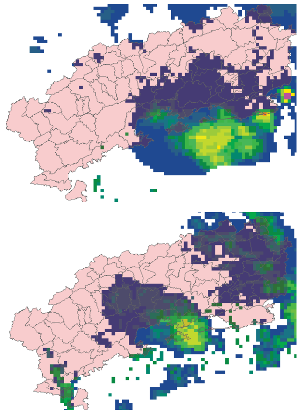
Fig. 4 - Precipitation grids in the state of Rio de Janeiro, Brazil, in 11 January 2011.
