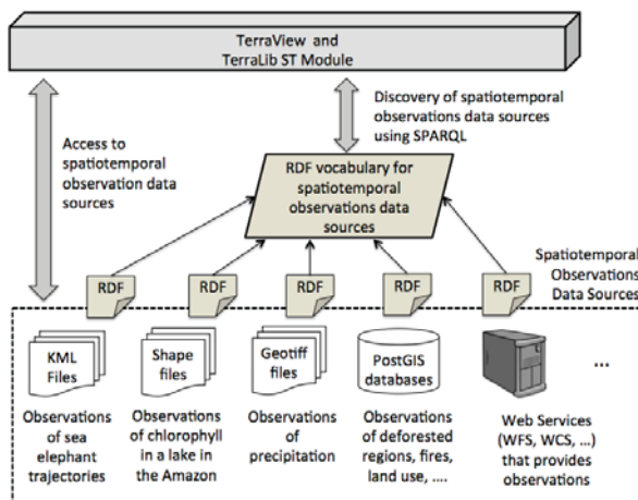
Fig. 7 - A proposal to access different kinds of spatiotemporal data sources.
