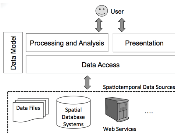
Fig. 5 - GIS general architecture.
