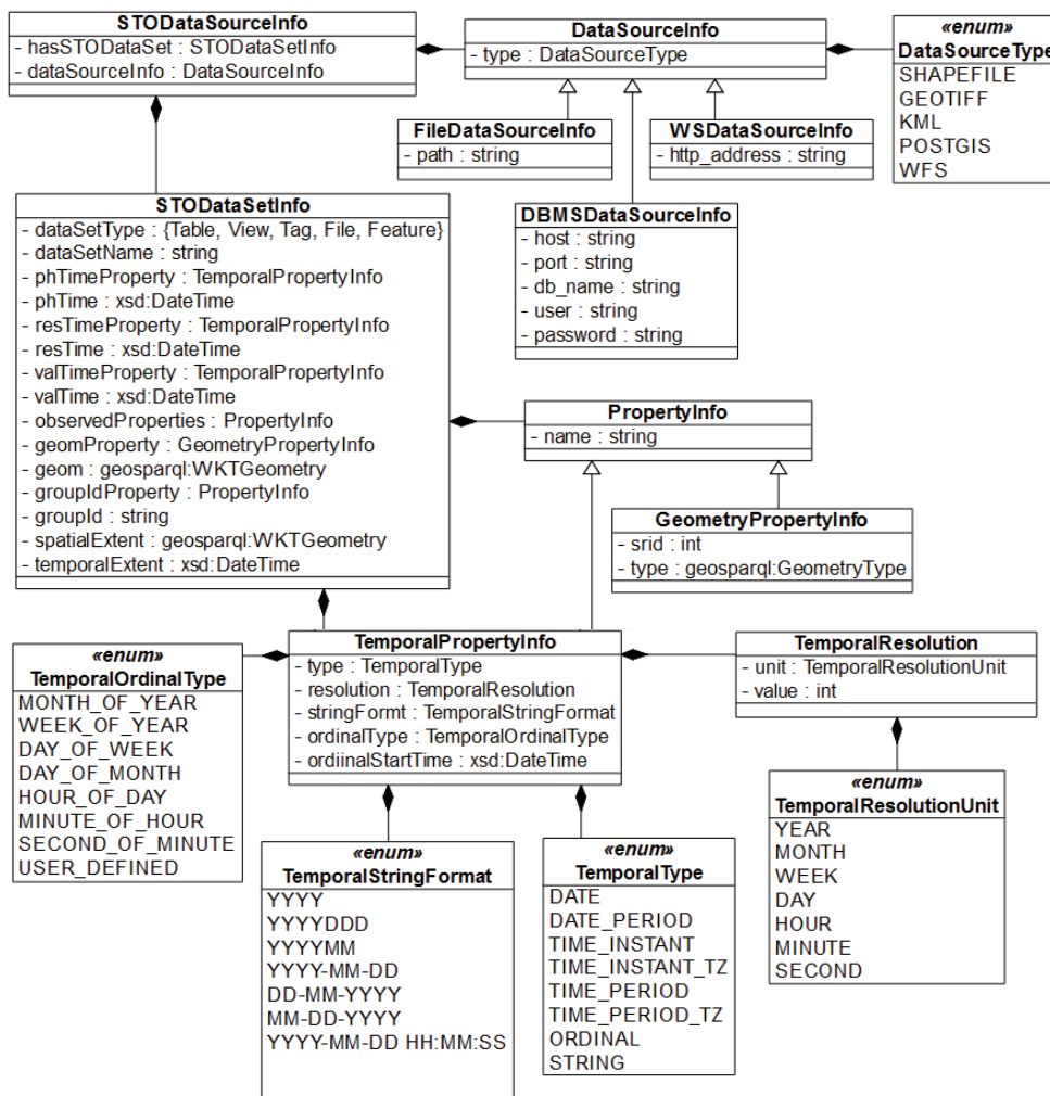
Fig. 8 - The RDF vocabulary for spatiotemporal observation data sources.
