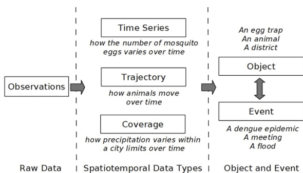
Fig. 6 - An Algebra for Spatiotemporal Data: From Observations To Events. Source: (Ferreira et al., 2014).
