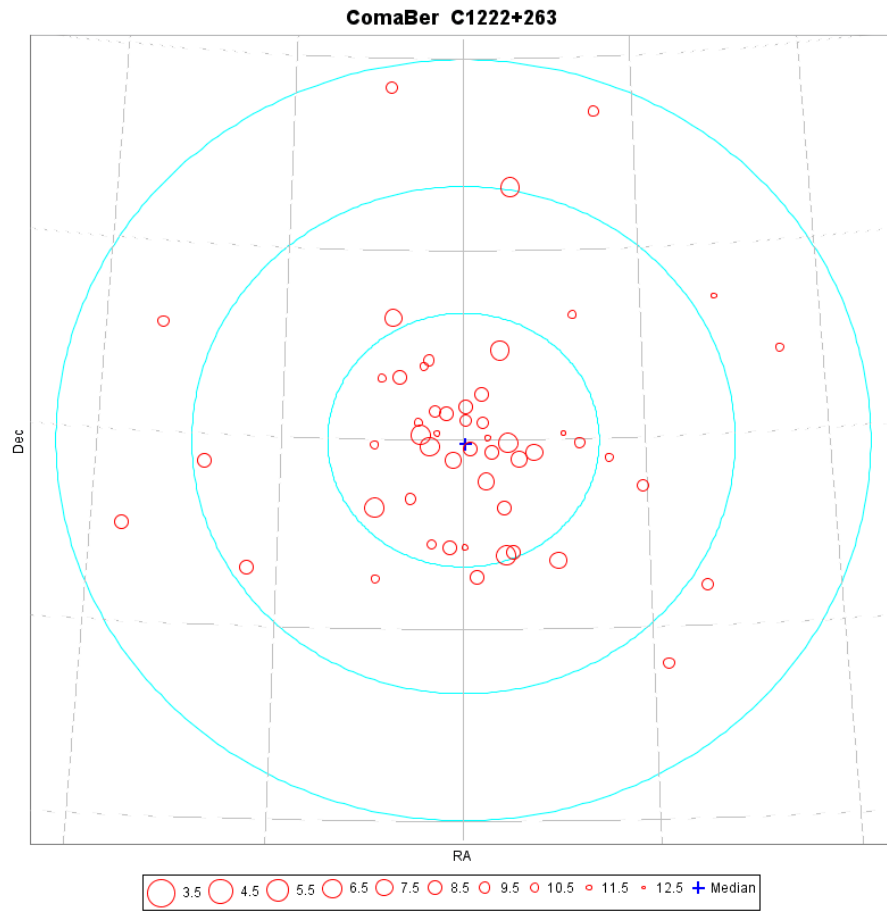
Fig. D.4. A map of members of the Coma Ber cluster as identified from the TGAS catalogue. The coordinate grid is at 5 degrees intervals, the three concentric circles are at 5, 10 and 15 pc from the cluster centre at the cluster distance.
