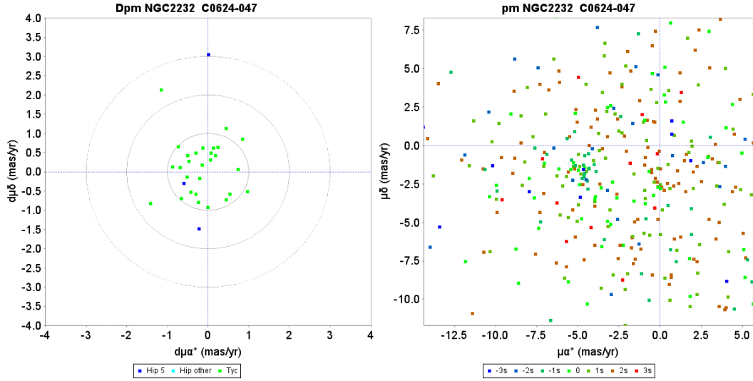
Fig. D.25. Proper motion charts for the cluster NGC2232. Left: unit weight residual proper motions. Green dots have first epoch Tycho -2 data, the dark blue dots have HIPPARCOS first epoch 5-parameter solutions. The concentric circles represent 1, 2, and 3 \sigma su levels. Right: actual proper motion distribution, where the colour indicate the difference from the cluster parallax in su units.
