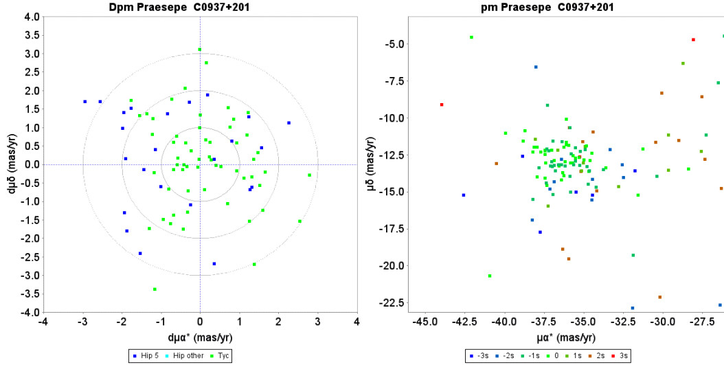
Fig. D.7. Proper motion charts for the Praesepe cluster. Left: unit weight residual proper motions. Green dots have first epoch Tycho -2 data, the dark blue dots have HIPPARCOS first epoch 5-parameter solutions. The concentric circles represent 1, 2, and 3 \sigma su levels. Right: actual proper motion distribution, where the colour indicate the difference from the cluster parallax in su units.
