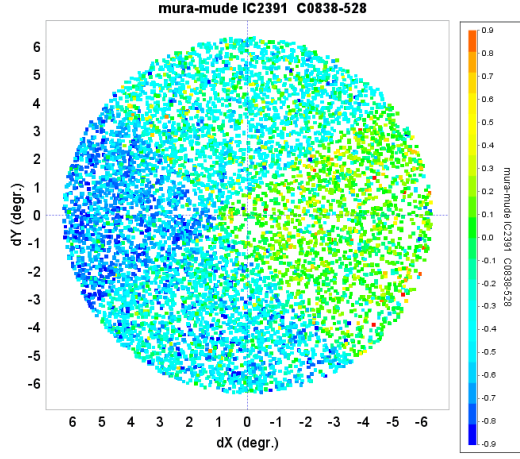
Fig. 28. Error correlations for the proper motion components in IC2391, for stars with Tycho-2 first epoch positions. The contributions of scans in different directions are clearly visible.
