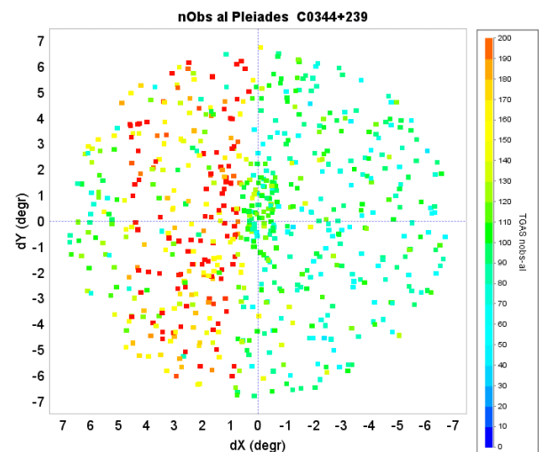
Fig. 2. The number of observations (CCD transits) per source in the TGAS catalogue for the Pleiades field. At this early stage there are still large local variations in the coverage. Positions are relative to the assumed centre of the Pleiades cluster. Each point represents a cluster or field star in the area.
