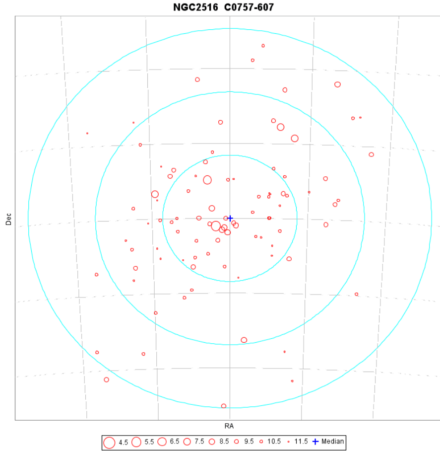
Fig. D.24. A map of members of the cluster NGC2516 as identified from the TGAS catalogue. The coordinate grid is at 1 degrees intervals, the three concentric circles are at 5, 10 and 15 pc from the cluster centre at the cluster distance.
