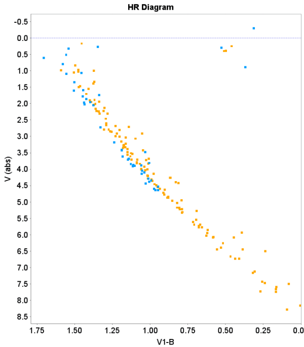
Fig. 15. The HR diagram for the Coma Berenices cluster (light blue) compared with the Hyades cluster (orange-red). Geneva photometry.
