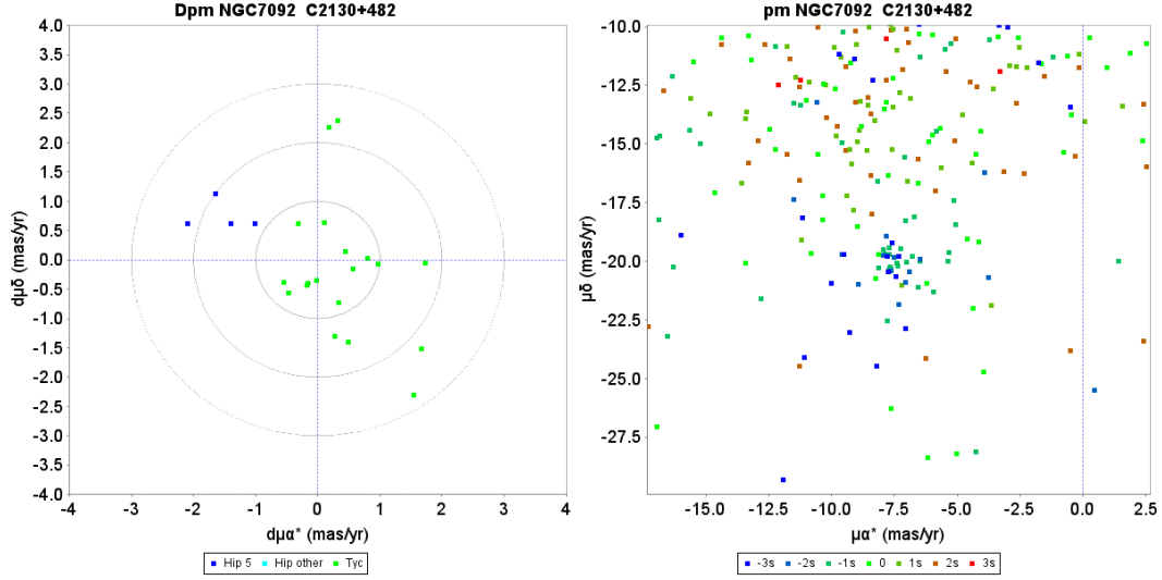
Fig. D.21. Proper motion charts for the cluster NGC7092. Left: unit weight residual proper motions. Green dots have first epoch Tycho -2 data, the dark blue dots have HIPPARCOS first epoch 5-parameter solutions. The concentric circles represent 1, 2, and 3 \sigma su levels. Right: actual proper motion distribution, where the colour indicate the difference from the cluster parallax in su units.
