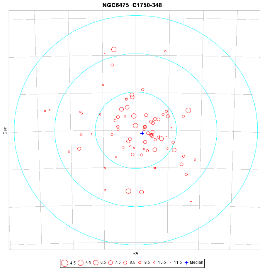
Fig. D.20. A map of members of the cluster NGC6475 as identified from the TGAS catalogue. The coordinate grid is at 1 degrees intervals, the three concentric circles are at 5, 10 and 15 pc from the cluster centre at the cluster distance.
