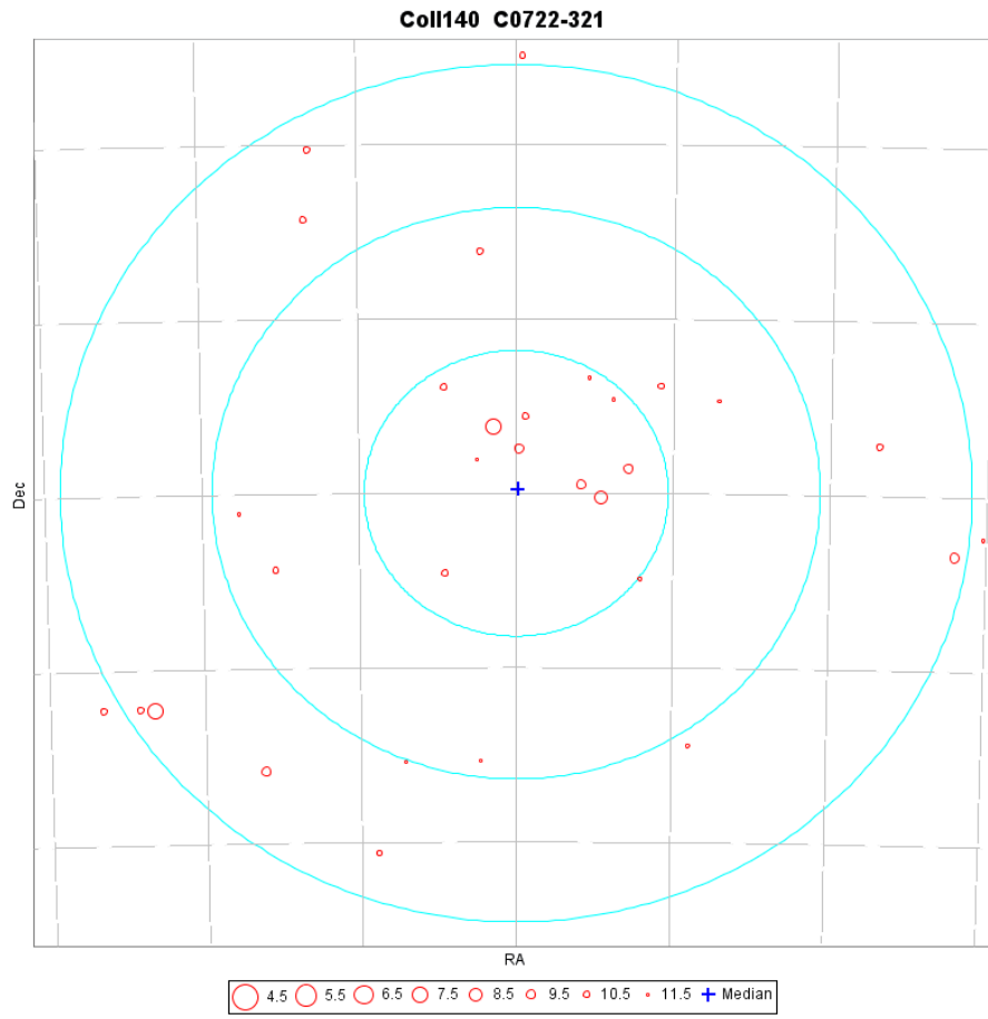
Fig. D.32. A map of members of the cluster Coll140 as identified from the TGAS catalogue. The coordinate grid is at 1 degrees intervals, the three concentric circles are at 5, 10 and 15 pc from the cluster centre at the cluster distance.
