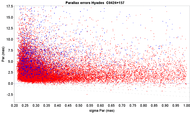
Fig. 6. The distribution of parallaxes as a function of su for stars in a field of 18 degrees radius centred on the Hyades cluster. The red and blue points as in Fig. 1. The three grey lines show the 1, 2 and 3\sigma su levels.
