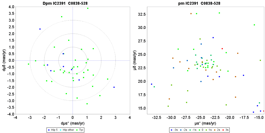
Fig. D.11. Proper motion charts for the cluster IC2391. Left: unit weight residual proper motions. Green dots have first epoch Tycho-2 data, the dark blue dots have HIPPARCOS first epoch 5-parameter solutions. The concentric circles represent 1, 2, and 3 \sigma su levels. Right: actual proper motion distribution, where the colour indicate the difference from the cluster parallax in su units.
