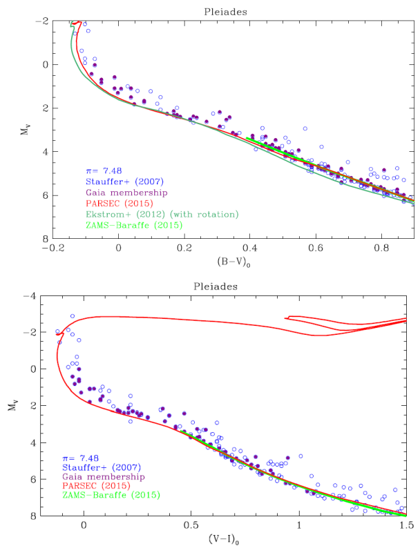
Fig. 25. M_V , (B-V)_0 HR diagram of the Pleiades, with several sets of commonly used isochrones (top). Filled dots: members confirmed with Gaia data; open dots: other cluster members. Bottom panel is the analogous in the M_V , (V-I)_0 . We assume an age of 130 Myr, solar metallicity, A_V=0.1 .
