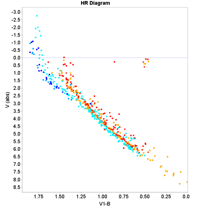
Fig. 30. The combined HR diagram for the Hyades and Praesepe (orange, red dots), Pleiades (light blue), IC2391 (blue) and IC 2602 (dark blue dots). Only data for astrometrically confirmed cluster members is shown. Geneva photometric data.
