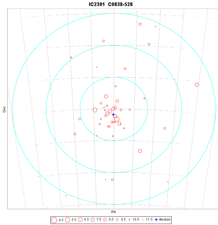
Fig. D.12. A map of members of the cluster IC2391 as identified from the TGAS catalogue. The coordinate grid is at 2 degrees intervals, the three concentric circles are at 5, 10 and 15 pc from the cluster centre at the cluster distance.
