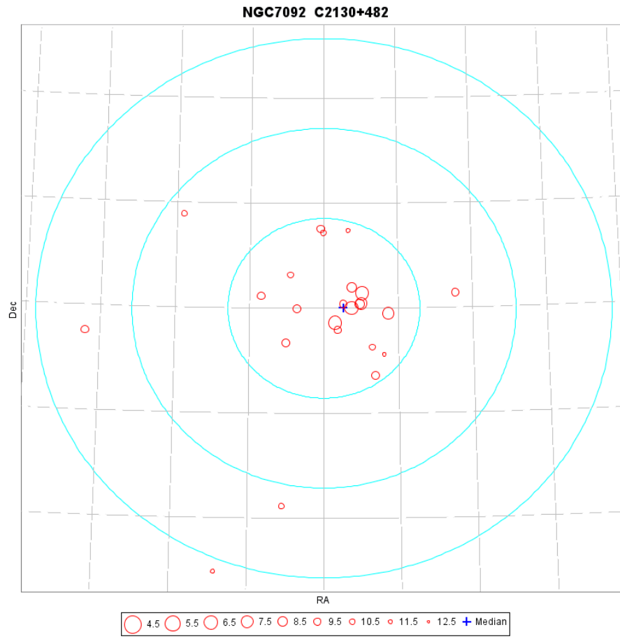
Fig. D.22. A map of members of the cluster NGC7092 as identified from the TGAS catalogue. The coordinate grid is at 1 degrees intervals, the three concentric circles are at 5, 10 and 15 pc from the cluster centre at the cluster distance.
