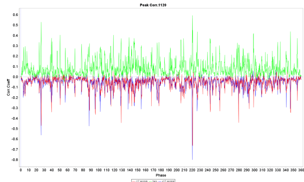
Fig. 5. An extract from the along-scan error correlations averaged over 20 satellite revolutions, against the rotation phase of the satellite. The green line shows the positive error correlations for sources separated by no more than 1 arcmin in transit phase (1 s in transit time). The red and blue lines show the error correlations for sources separated by \pm 17 arcmin respectively. All of the larger peaks can be related to clanks, and can be observed as such in a reconstruction of the satellite spin rate.
