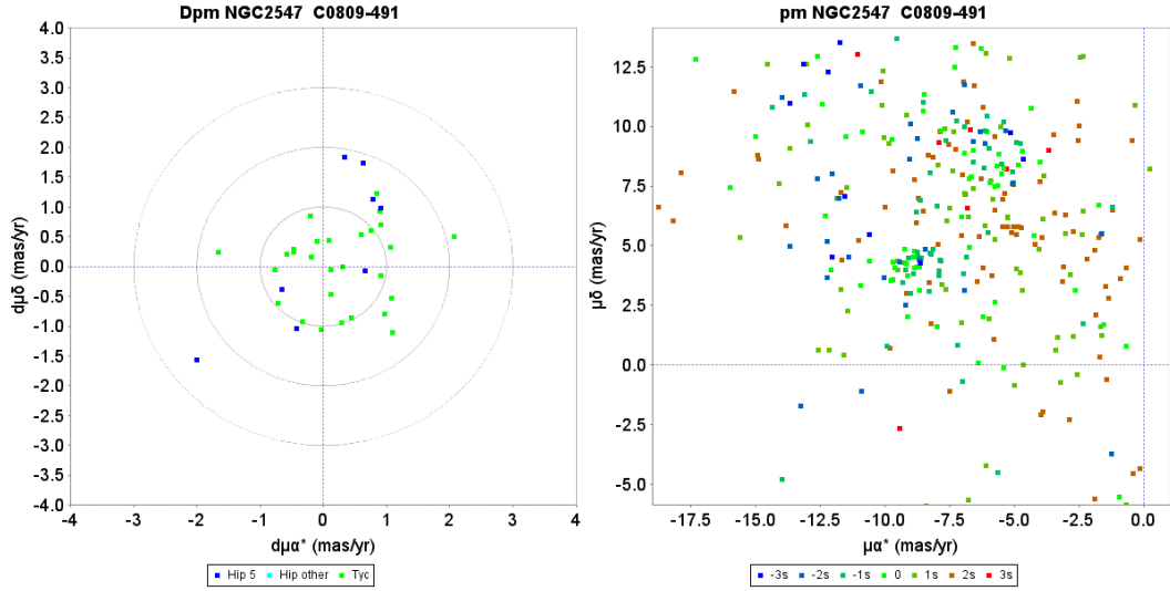
Fig. D.37. Proper motion charts for the cluster NGC2547. Left: unit weight residual proper motions. Green dots have first epoch Tycho-2 data, the dark blue dots have HIPPARCOS first epoch 5-parameter solutions. The concentric circles represent 1, 2, and 3\sigma su levels. Right: actual proper motion distribution, where the colour indicate the difference from the cluster parallax in su units.
