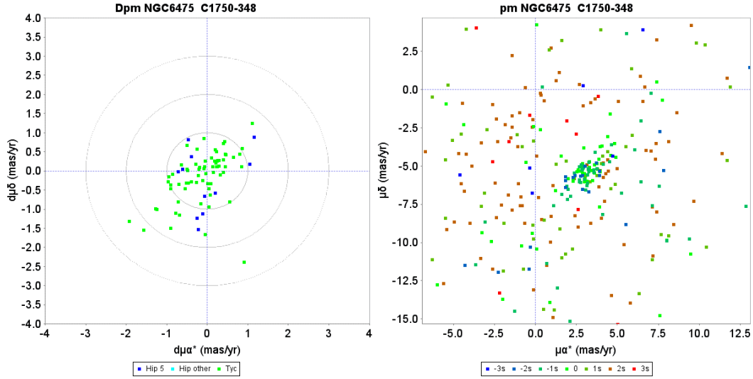
Fig. D.19. Proper motion charts for the cluster NGC6475. Left: unit weight residual proper motions. Green dots have first epoch Tycho -2 data, the dark blue dots have HIPPARCOS first epoch 5-parameter solutions. The concentric circles represent 1, 2, and 3 \sigma su levels. Right: actual proper motion distribution, where the colour indicate the difference from the cluster parallax in su units.
