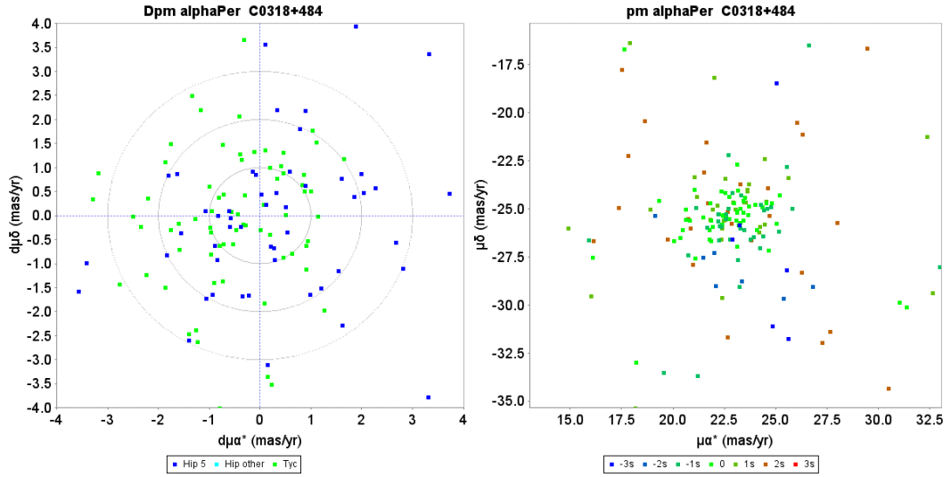
Fig. D.9. Proper motion charts for the \alpha Per cluster. Left: unit weight residual proper motions. Green dots have first epoch Tycho -2 data, the dark blue dots have HIPPARCOS first epoch 5-parameter solutions. The concentric circles represent 1, 2, and 3 \sigma su levels. Right: actual proper motion distribution, where the colour indicate the difference from the cluster parallax in su units.
