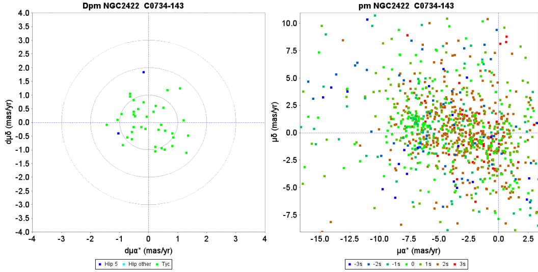
Fig. D.33. Proper motion charts for the cluster NGC2422. Left: unit weight residual proper motions. Green dots have first epoch Tycho-2 data, the dark blue dots have HIPPARCOS first epoch 5-parameter solutions. The concentric circles represent 1, 2, and 3 \sigma su levels. Right: actual proper motion distribution, where the colour indicate the difference from the cluster parallax in su units.
