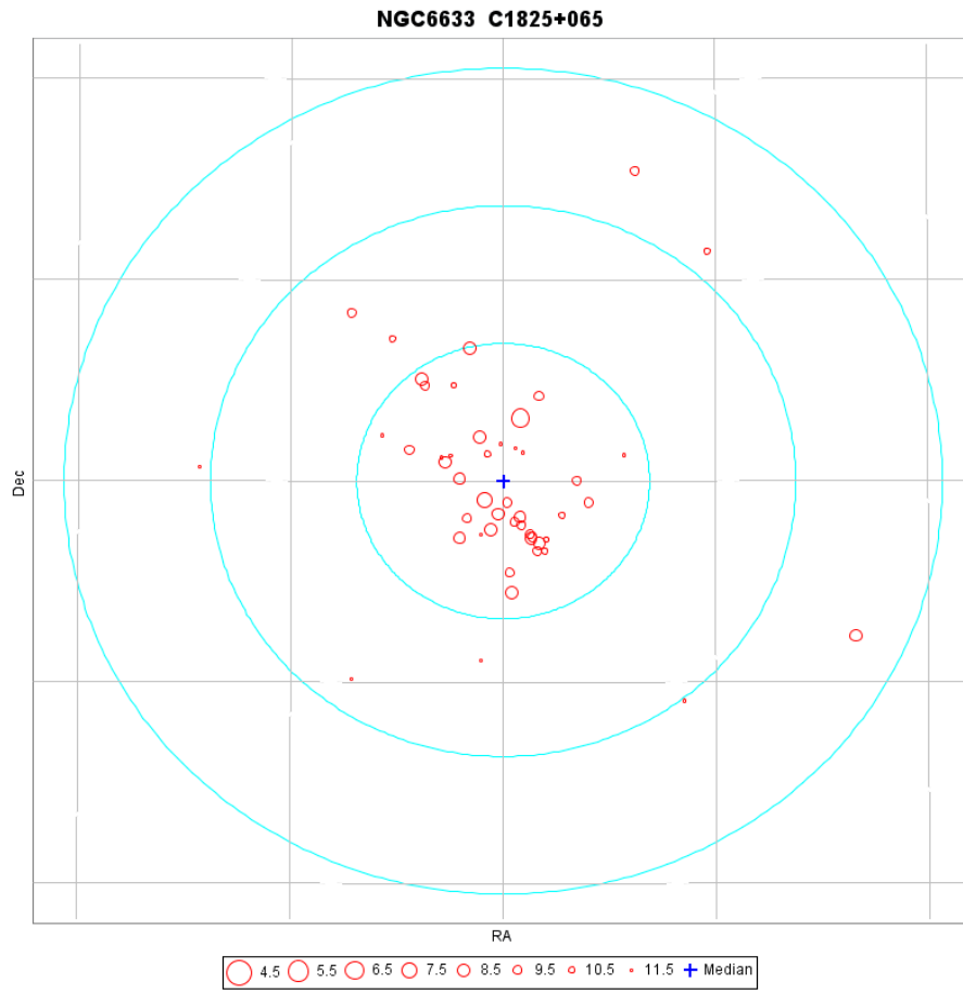
Fig. D.30. A map of members of the cluster NGC6633 as identified from the TGAS catalogue. The coordinate grid is at 1 degrees intervals, the three concentric circles are at 5, 10 and 15 pc from the cluster centre at the cluster distance.
