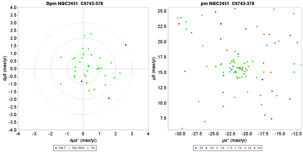
Fig. D.17. Proper motion charts for the cluster NGC2451. Left: unit weight residual proper motions. Green dots have first epoch Tycho -2 data, the dark blue dots have HIPPARCOS first epoch 5-parameter solutions. The concentric circles represent 1, 2, and 3 \sigma su levels. Right: actual proper motion distribution, where the colour indicate the difference from the cluster parallax in su units.
