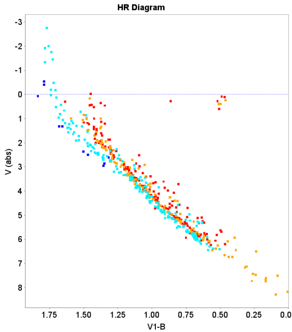
Fig. 32. The combined HR diagrams for the Hyades and Praesepe (orange, red), Pleiades (light blue) and confirmed members of NGC2451A (dark blue), in Geneva photometry.
