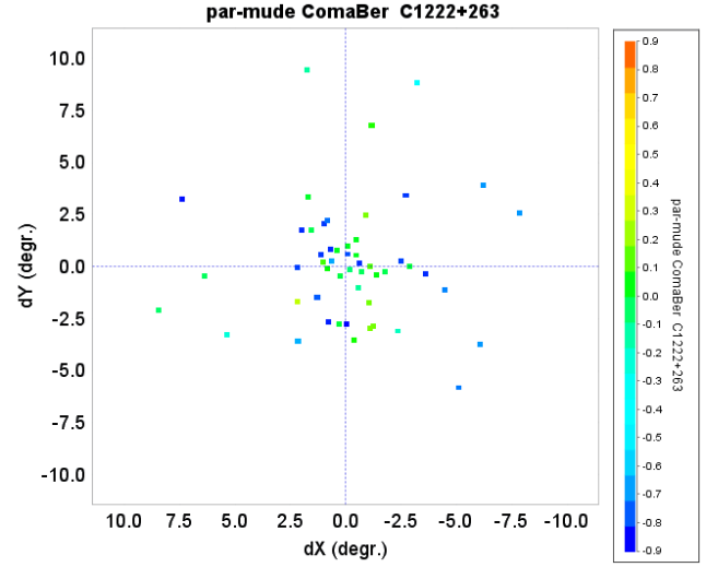
Fig. 14. The stars in the Coma Berenice cluster, colour coded according to the error-correlations between the parallax and proper motion in declination. The dark blue dots, representing strong negative error correlations, have first epoch Tycho-2 data, the green dots, representing near-zero correlations, have first epoch HIPPARCOS data.
