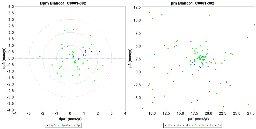
Fig. D.15. Proper motion charts for the cluster Blanco 1. Left: unit weight residual proper motions. Green dots have first epoch Tycho -2 data, the dark blue dots have HIPPARCOS first epoch 5-parameter solutions. The concentric circles represent 1, 2, and 3 \sigma su levels. Right: actual proper motion distribution, where the colour indicate the difference from the cluster parallax in su units.
