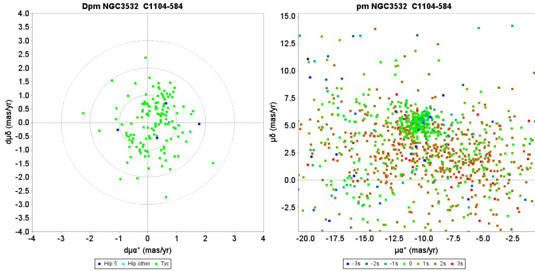
Fig. D.35. Proper motion charts for the cluster NGC3532. Left: unit weight residual proper motions. Green dots have first epoch Tycho -2 data, the dark blue dots have HIPPARCOS first epoch 5-parameter solutions. The concentric circles represent 1, 2, and 3 \sigma su levels. Right: actual proper motion distribution, where the colour indicate the difference from the cluster parallax in su units.
