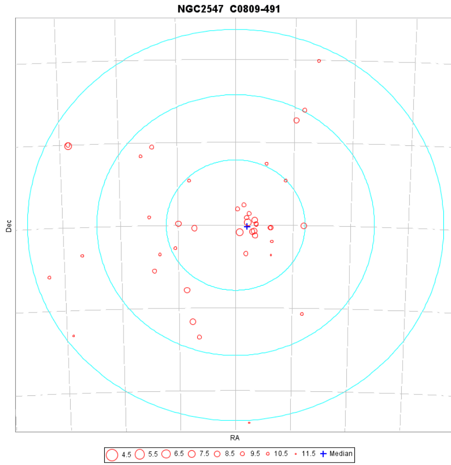
Fig. D.38. A map of members of the cluster NGC2547 as identified from the TGAS catalogue. The coordinate grid is at 0.5 degrees intervals, the three concentric circles are at 5, 10 and 15 pc from the cluster centre at the cluster distance.
