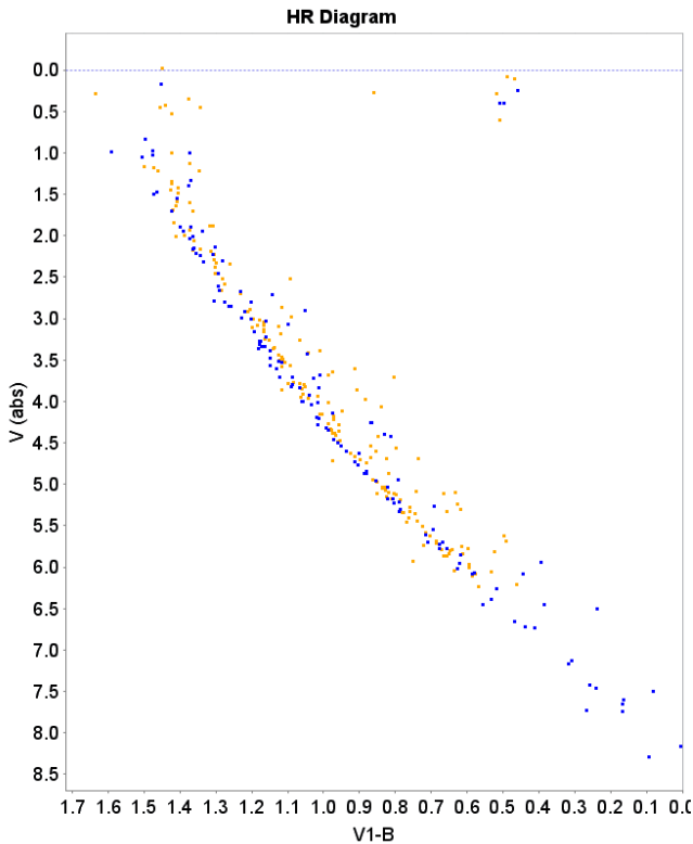
Fig. 18. The HR diagram in Geneva photometry for the Hyades (blue dots) and Praesepe (orange dots) clusters. For the Hyades stars individual kinematically improved parallaxes were used, for the Praesepe stars the common cluster parallax. As was also observed in fv109, the two main sequences accurately coincide.
