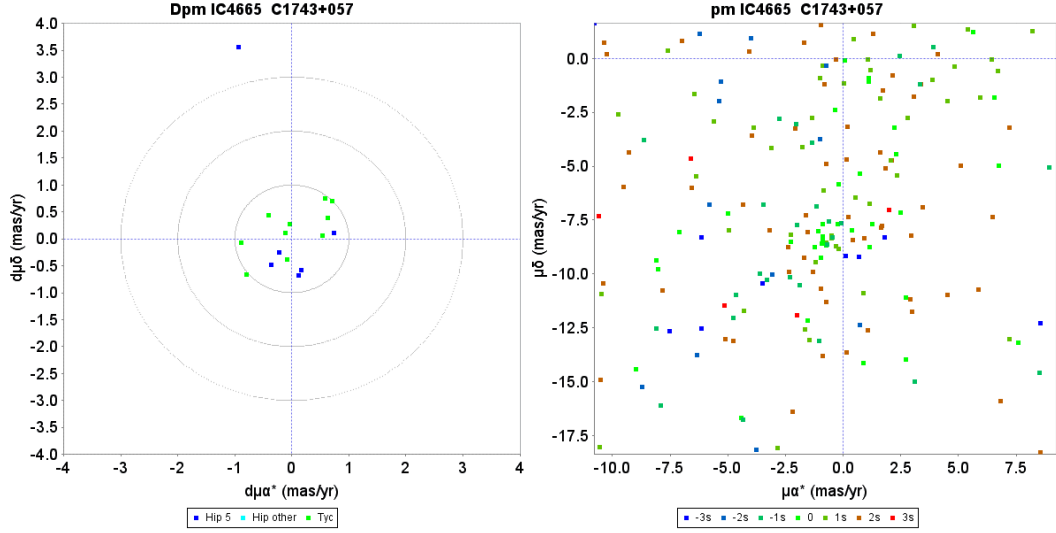
Fig. D.27. Proper motion charts for the cluster IC4665. Left: unit weight residual proper motions. Green dots have first epoch Tycho -2 data, the dark blue dots have HIPPARCOS first epoch 5-parameter solutions. The concentric circles represent 1, 2, and 3 \sigma su levels. Right: actual proper motion distribution, where the colour indicate the difference from the cluster parallax in su units.
