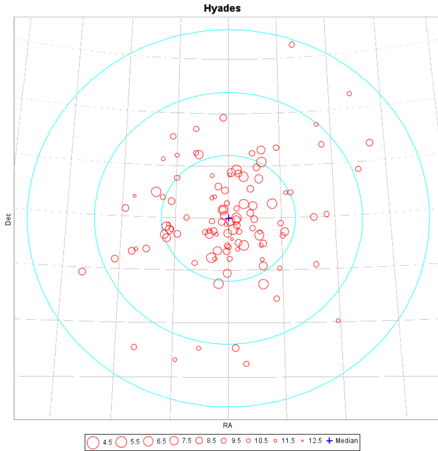
Fig. D.2. A map of the Hyades members as identified from the TGAS catalogue. The coordinate grid is at 5 degrees intervals, the three concentric circles are at 5, 10 and 15 pc from the cluster centre at the cluster distance.
