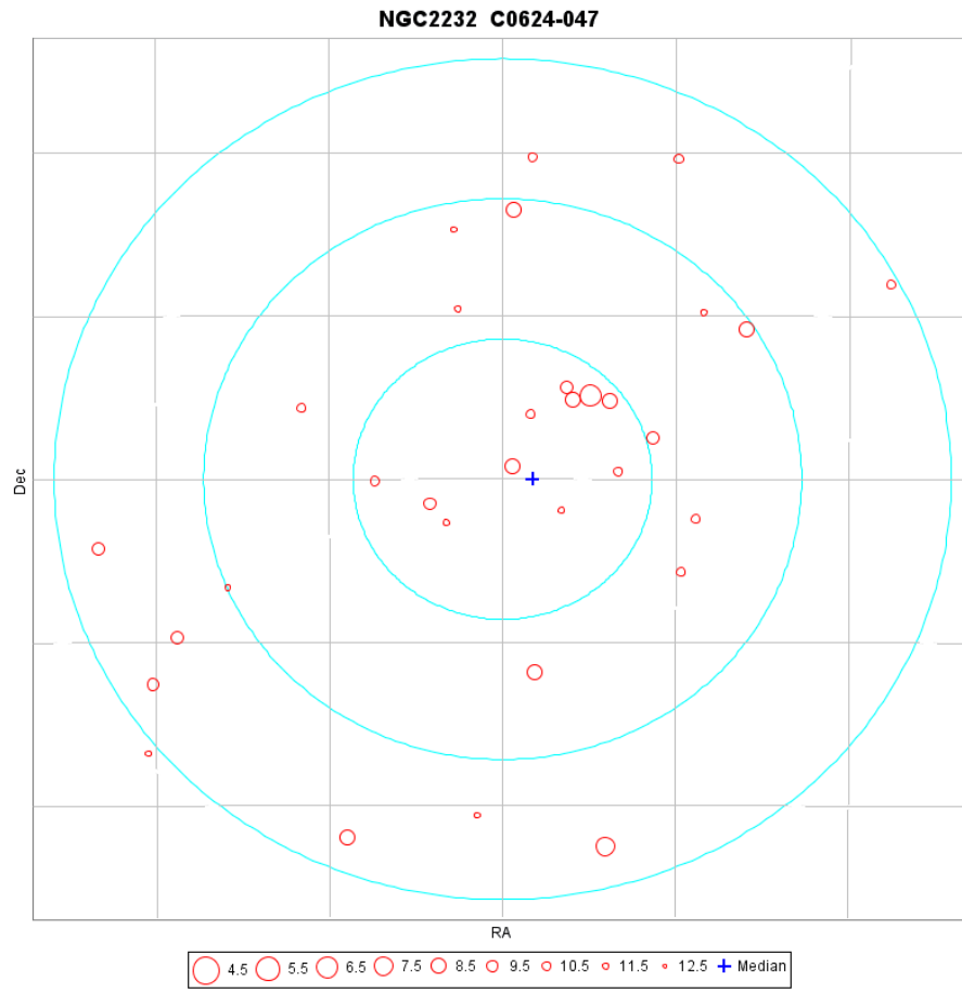
Fig. D.26. A map of members of the cluster NGC2232 as identified from the TGAS catalogue. The coordinate grid is at 1 degrees intervals, the three concentric circles are at 5, 10 and 15 pc from the cluster centre at the cluster distance.
