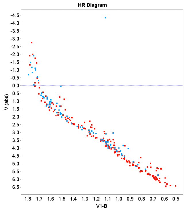
Fig. 27. The Geneva photometry HR diagram for the \alpha Per cluster (blue dots) compared with the data on the Pleiades cluster (red dots). Reddening corrections were applied for both clusters. Geneva photometry.
