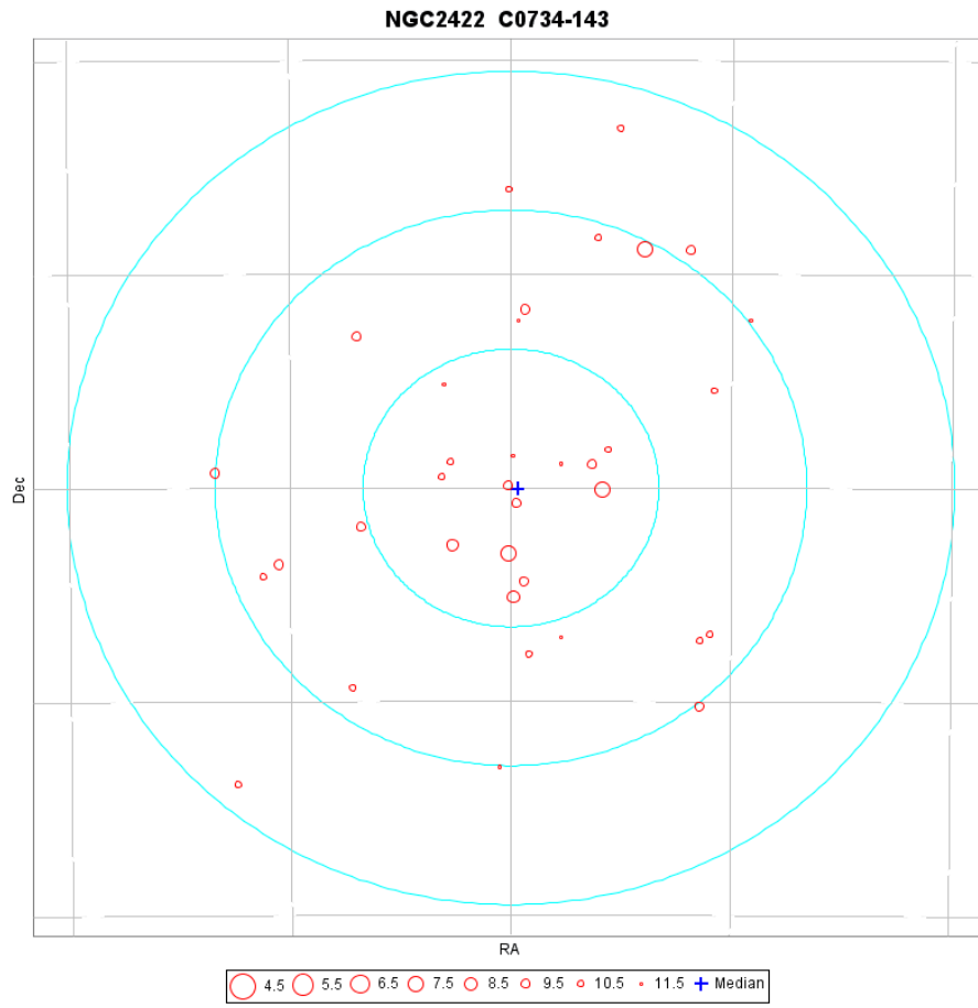
Fig. D.34. A map of members of the cluster NGC2422 as identified from the TGAS catalogue. The coordinate grid is at 1 degrees intervals, the three concentric circles are at 5, 10 and 15 pc from the cluster centre at the cluster distance.
