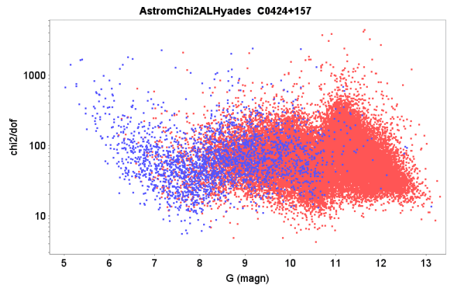
Fig. 1. This diagram shows the logarithm of the square root of the normalized \chi^2 values for the astrometric solutions as a function of the G -band magnitude. The data come from an 18 degrees radius field, centred on the Hyades cluster. The blue dots used first epoch from the HIPPARCOS catalogue, the red dots from the Tycho-2 catalogue.
