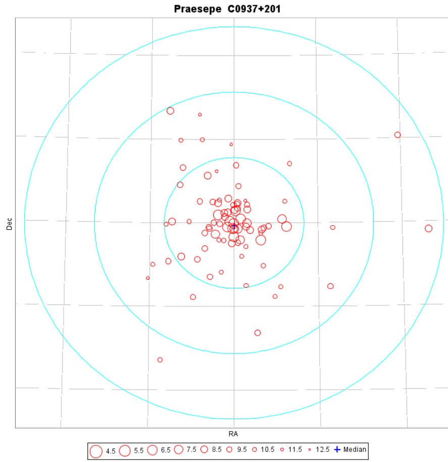
Fig. D.8. A map of members of the Praesepe cluster as identified from the TGAS catalogue. The coordinate grid is at 2 degrees intervals, the three concentric circles are at 5, 10 and 15 pc from the cluster centre at the cluster distance.
