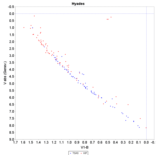
Fig. 13. The absolute magnitudes and colour indices in the Geneva photometry for cluster members, after applying distance moduli based on individual kinematically improved parallaxes. The red dots represent stars not present in the TGAS catalogue, but with similarly treated data in fv109 .
