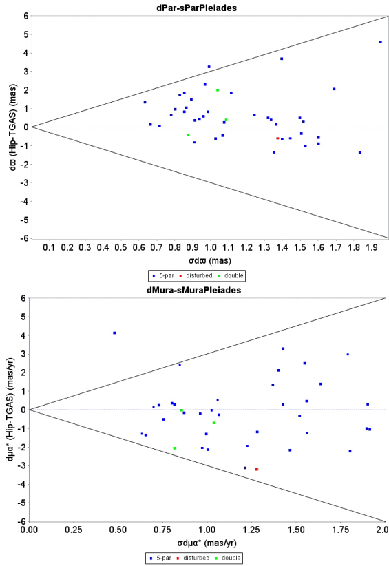
Fig. 21. Differences in parallax (top) and proper motion in Right Ascension (bottom) between the HIPPARCOS and TGAS solutions, for members of the Pleiades cluster, and as a function of the errors on the differences.
