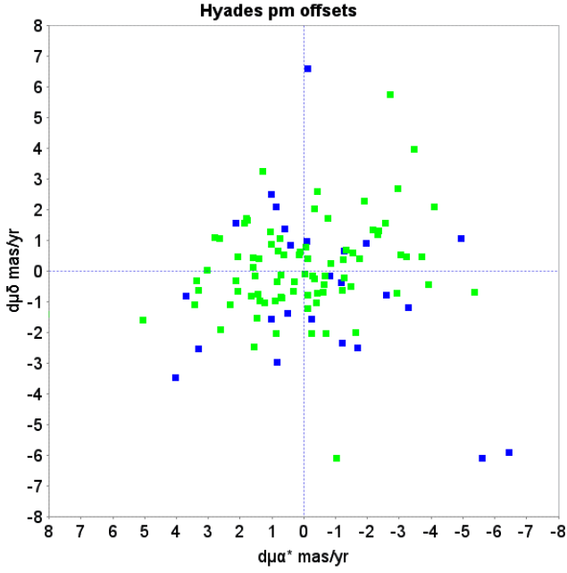
Fig. 10. Differences between predicted and observed proper motions for stars within the space volume of the Hyades cluster, showing the results for 112 possible members. Green dots: First epoch HIPPARCOS; blue dots: first epoch Tycho-2.
