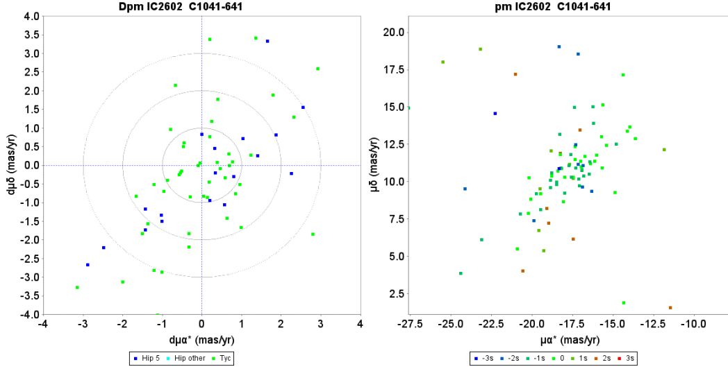
Fig. D.13. Proper motion charts for the cluster IC2602. Left: unit weight residual proper motions. Green dots have first epoch Tycho-2 data, the dark blue dots have HIPPARCOS first epoch 5-parameter solutions. The concentric circles represent 1, 2, and 3 \sigma su levels. Right: actual proper motion distribution, where the colour indicate the difference from the cluster parallax in su units.
