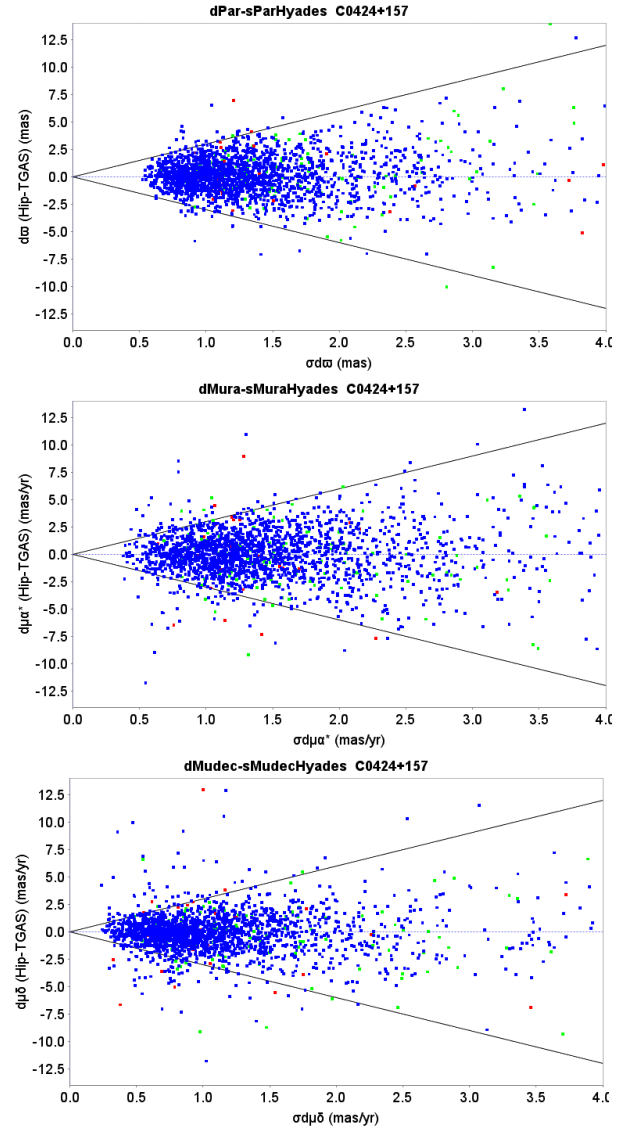
Fig. 8. Differences in astrometric parameters as a function of the su of the differences between the HIPPARCOS and TGAS solutions for stars, as measured in a field of 18^\circ radius centred on the Hyades cluster. The blue dots represent clean 5-parameter solutions in the HIPPARCOS data. The red dots represent primarily accelerated solutions (so-called 7 and 9 parameter solutions). The green dots were solved as double stars in the HIPPARCOS solution. The two black lines show the \pm 3\sigma su levels. From top to bottom: Parallaxes, proper motions in right ascension, proper motion in declination.
