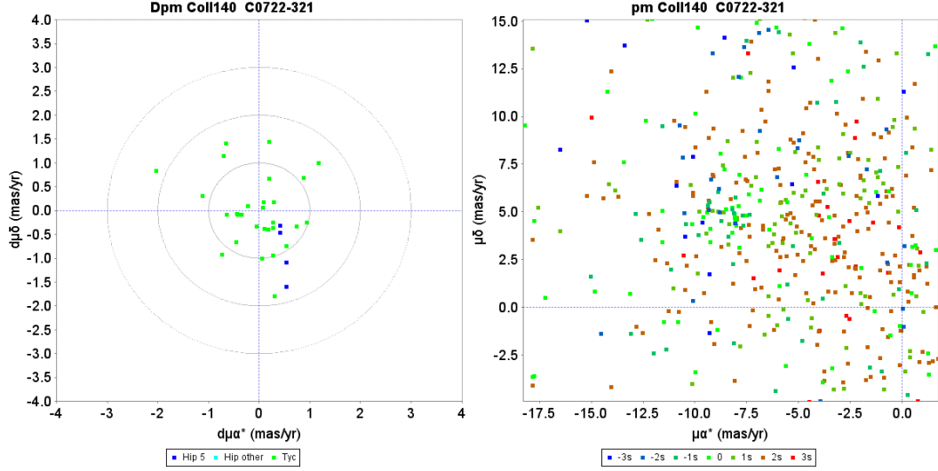
Fig. D.31. Proper motion charts for the cluster Coll140. Left: unit weight residual proper motions. Green dots have first epoch Tycho -2 data, the dark blue dots have HIPPARCOS first epoch 5-parameter solutions. The concentric circles represent 1, 2, and 3 \sigma su levels. Right: actual proper motion distribution, where the colour indicate the difference from the cluster parallax in su units.
