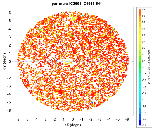
Fig. 29. Error correlations between the parallax and proper motion in Right Ascension in the field of IC2602, for stars with first epoch positions from the Tycho-2 catalogue.
