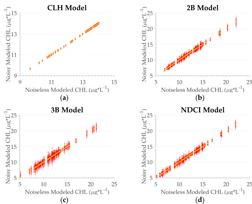
Figure 6. Algorithm performance for the chl-a concentration of the OLCI sensor. (a) CLH; (b) 2B; (c) 3B; (d) NDCI. Circles in red represent the data with noise, circles in yellow the noiseless data. The transparency is based on the frequency distribution, in which opaque indicates a higher frequency, and transparent indicates a lower frequency.
