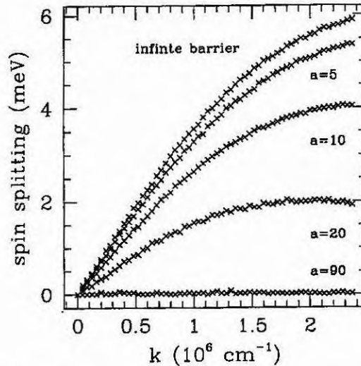
Figure 2. Splittings obtained with the asymmetric potential well in equation (7). The bulk parameters are those of InAs and V_0 = 400 meV. We have set b = 100\text{\AA} and plotted the results for different values of a in \text{\AA} . The solution with an infinite barrier at z = 0 is also shown.
