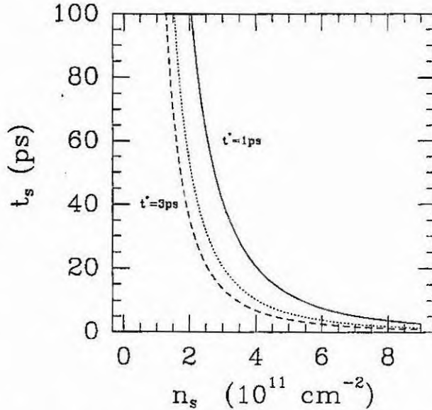
Figure 4. Average D'yakonov-Perel electron spin relaxation time t_s at the Fermi "surface" of an AlGaAs/GaAs hetero- junction with varying carrier concentration n_s . We have used a = 0.5 = 17\text{eV } \text{\AA}^3 and varied t^* between 1 and 3 ps.
