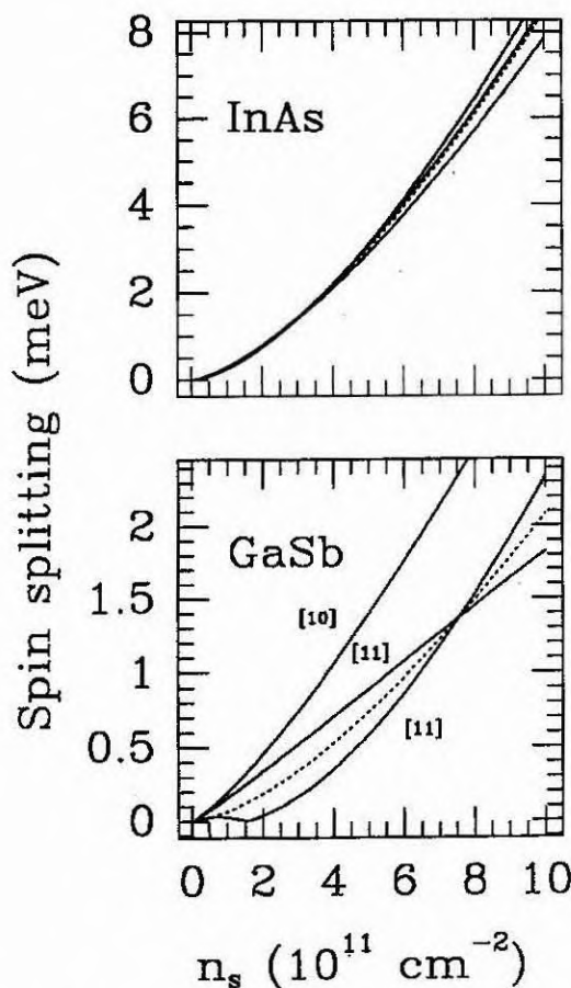
Figure 1. Spin-orbit splitting at three points of the Fermi "surface" along different directions in k -space (indicated in the case of GaSb), as a function of the carrier density n_s . The dashed line gives the isotropic contribution of the Rashba term alone. Only the first subband is occupied.
